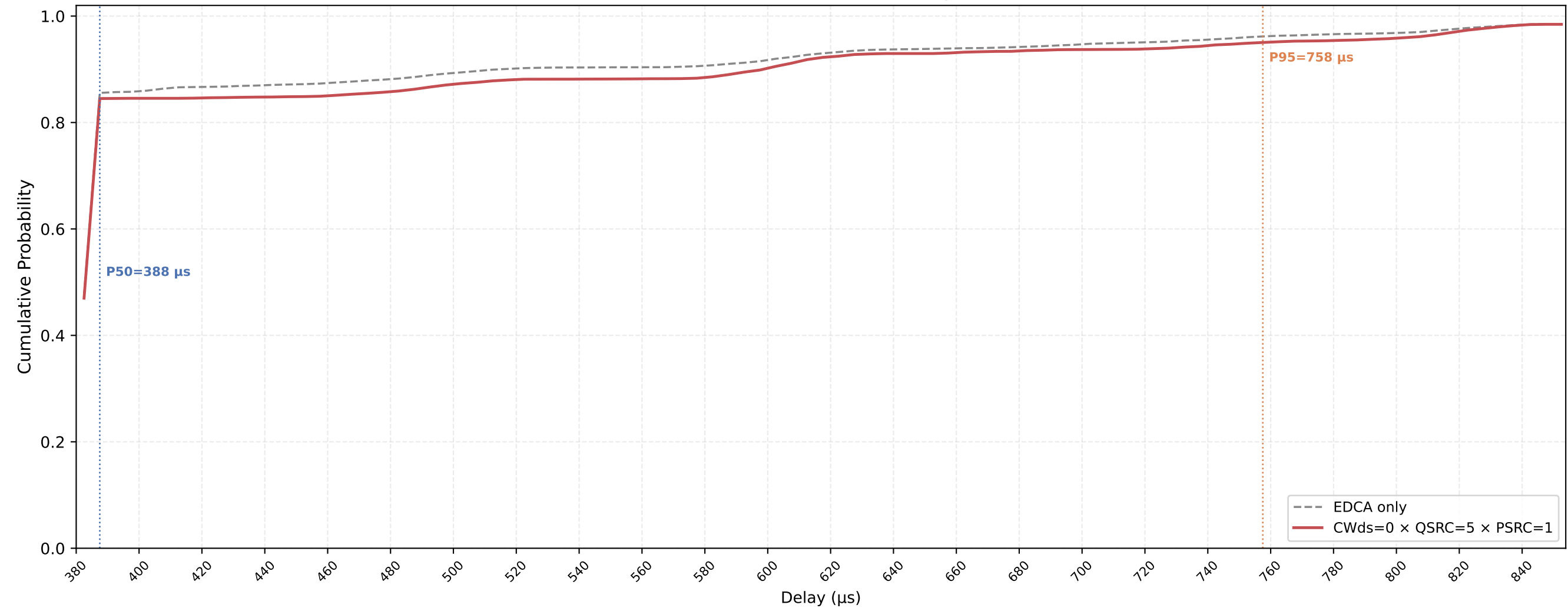
Legacy STA VO Delay CDF — CWds=0 × QSRC=5 × PSRC=1 nSta=30, nPedca=15, 0.1Mbps, avg of 10 runs
