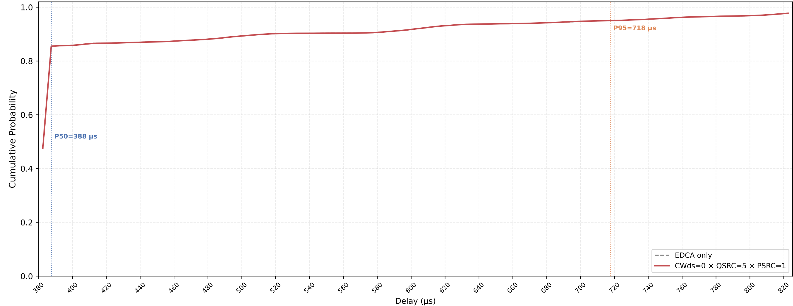
P-EDCA STA VO Delay CDF — CWds=0 × QSRC=5 × PSRC=1 nSta=30, nPedca=30, 0.1Mbps, avg of 10 runs
