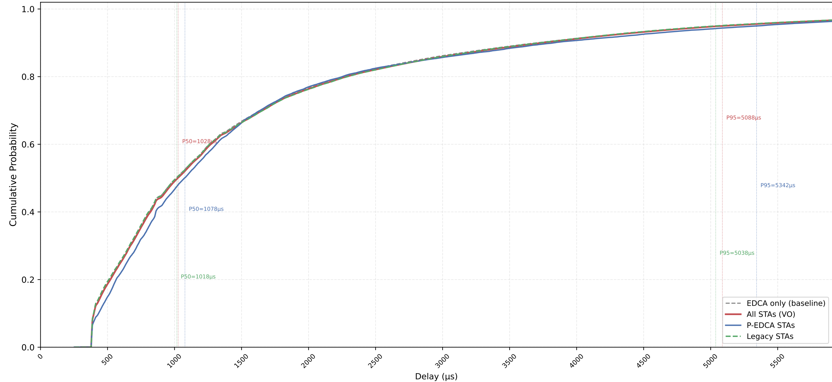
VO Delay CDF — P-EDCA / Legacy / All | CWds=0 × QSRC=5 × PSRC=2 nSta=30, nPedca=5/30, 0.5Mbps, avg of 10 runs
