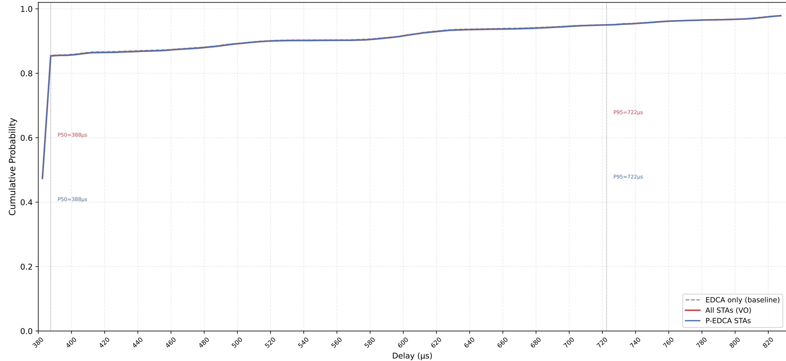
VO Delay CDF — P-EDCA / Legacy / All | CWds=0 × QSRC=5 × PSRC=2 nSta=30, nPedca=30/30, 0.1Mbps, avg of 10 runs
