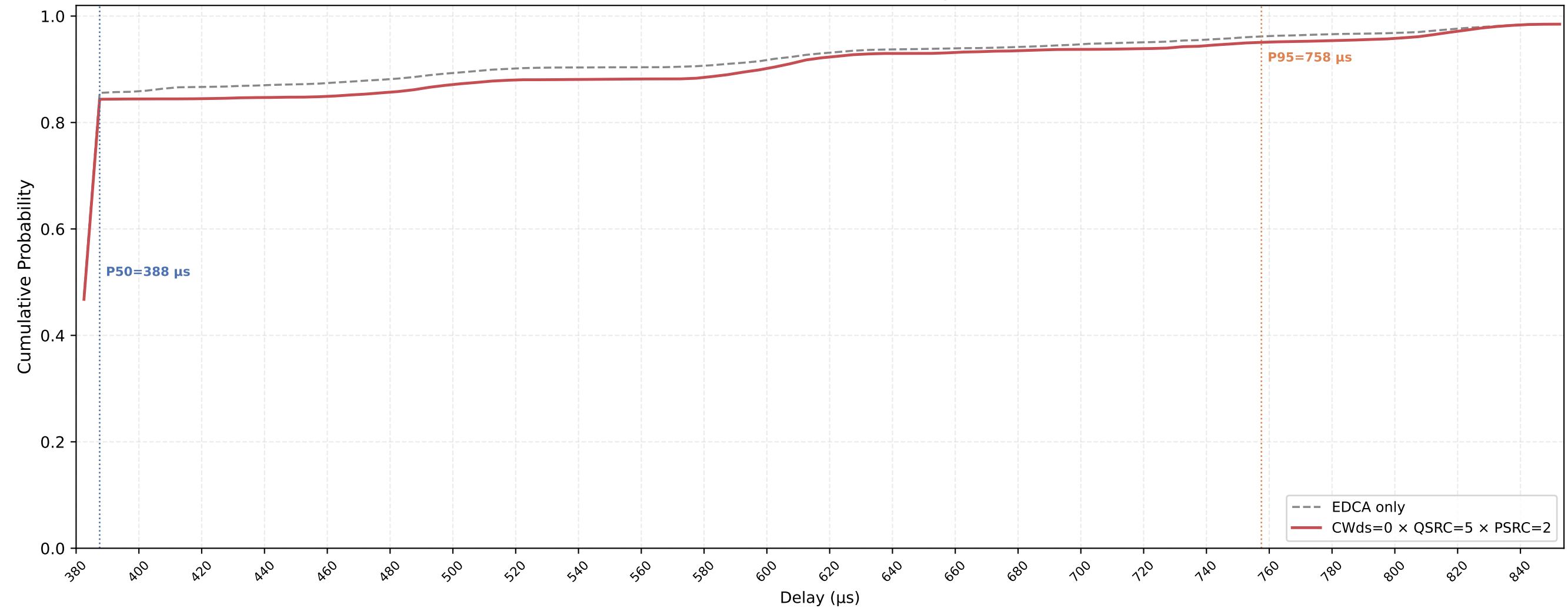
Legacy STA VO Delay CDF — CWds=0 × QSRC=5 × PSRC=2 nSta=30, nPedca=15, 0.1Mbps, avg of 10 runs
