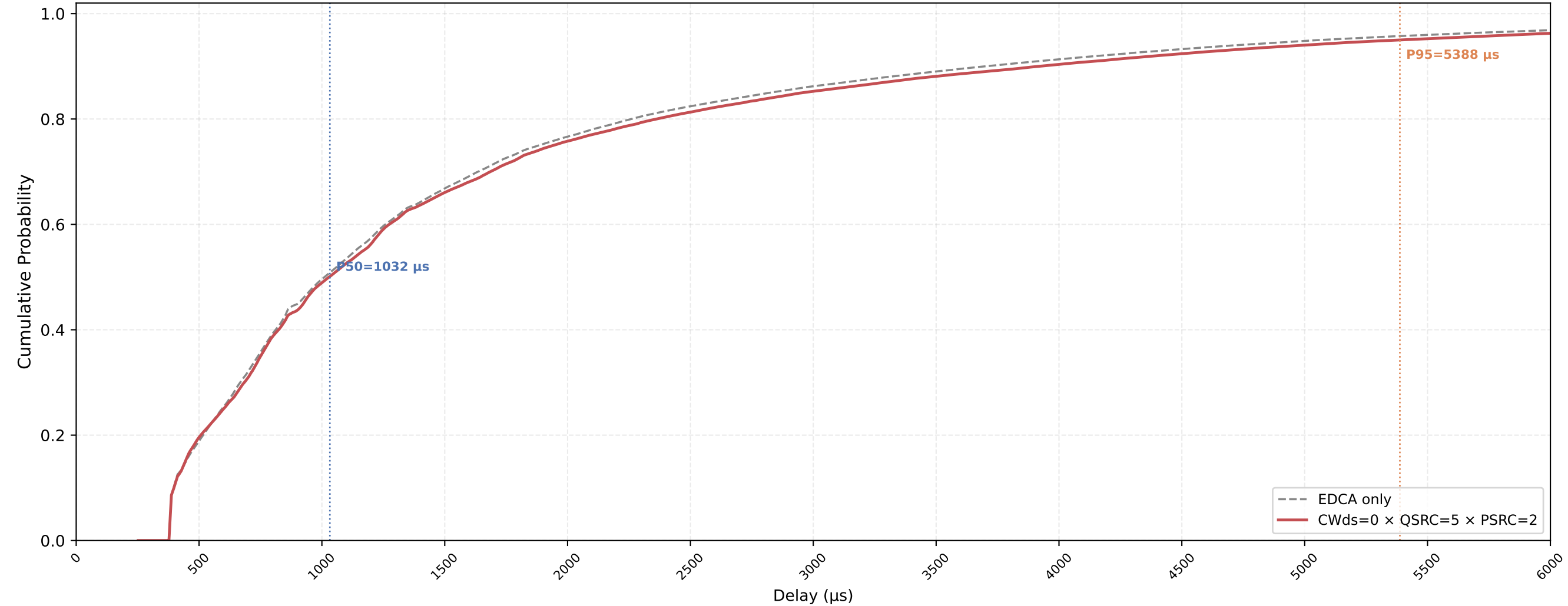
Legacy STA VO Delay CDF — CWds=0 × QSRC=5 × PSRC=2 nSta=30, nPedca=15, 0.5Mbps, avg of 10 runs
