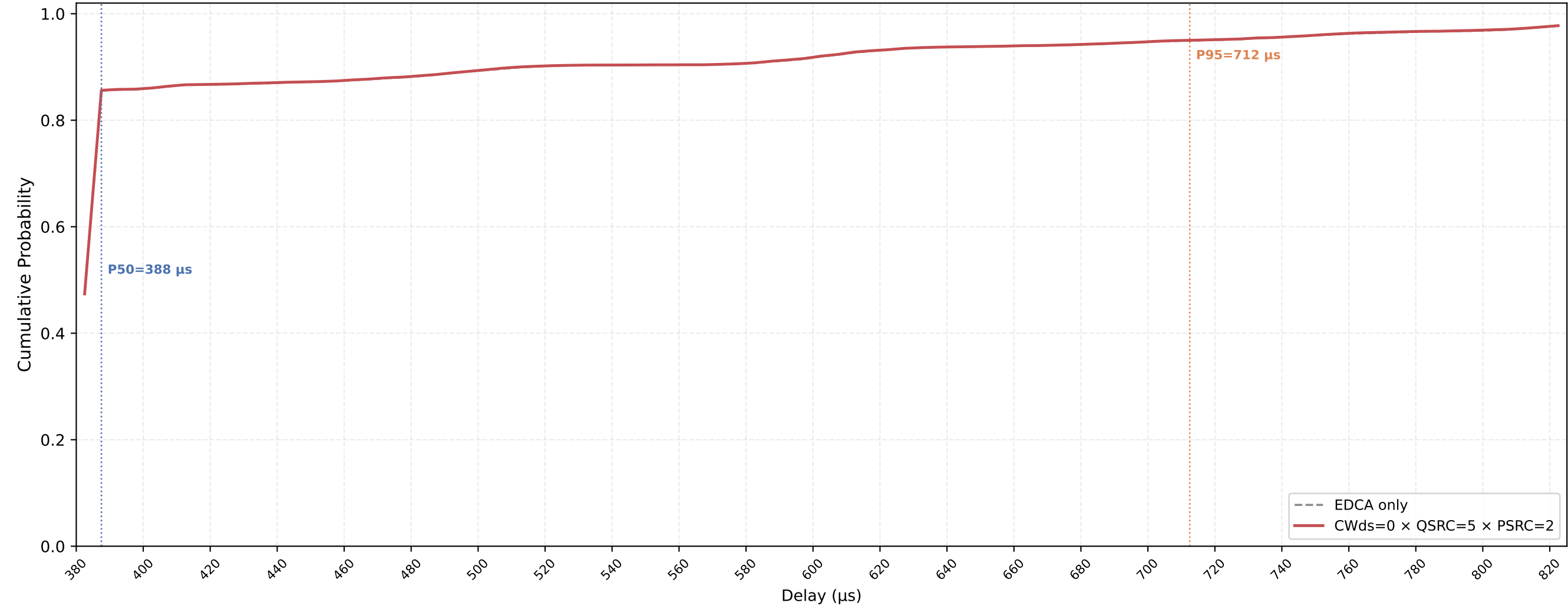
VO (all STAs) Delay CDF — CWds=0 × QSRC=5 × PSRC=2 nSta=30, nPedca=5, 0.1Mbps, avg of 10 runs
