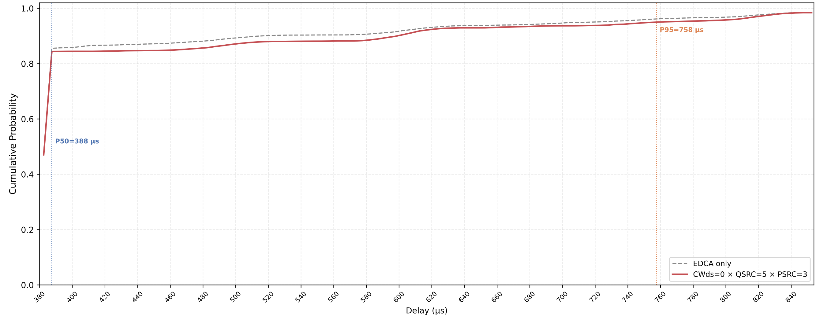
Legacy STA VO Delay CDF — CWds=0 × QSRC=5 × PSRC=3 nSta=30, nPedca=15, 0.1Mbps, avg of 10 runs
