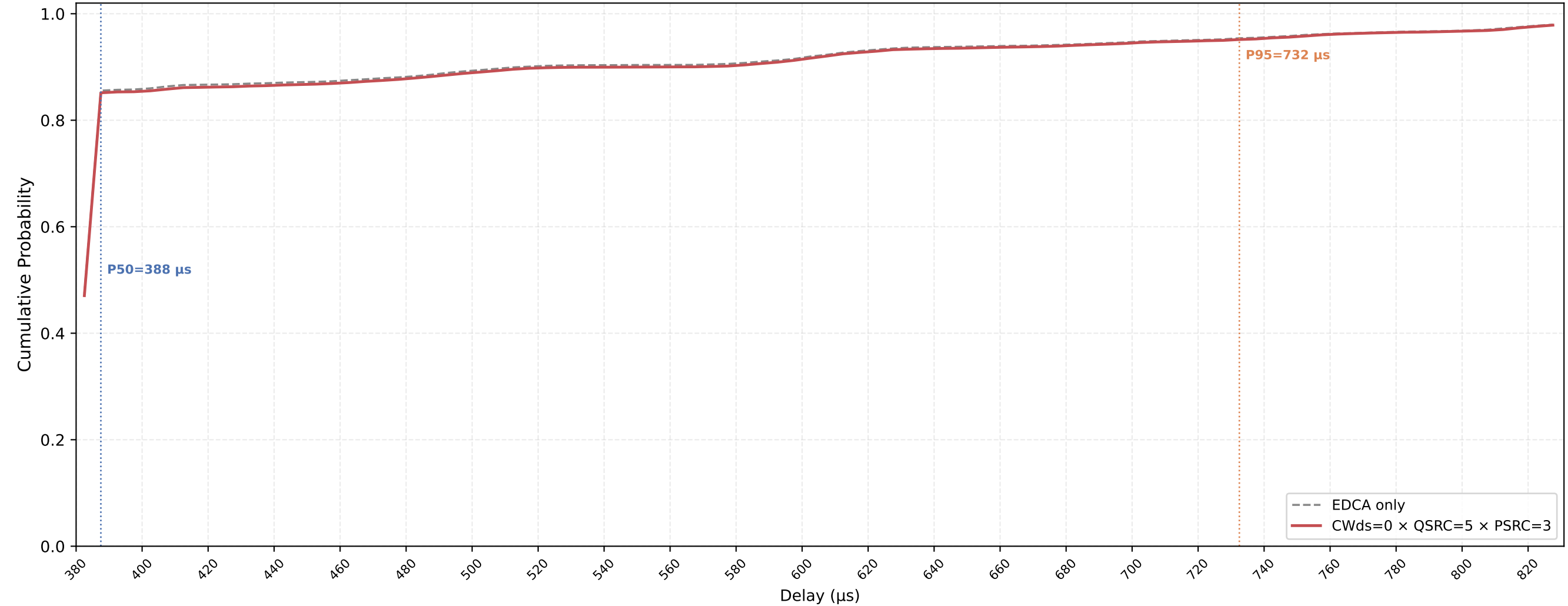
VO (all STAs) Delay CDF — CWds=0 × QSRC=5 × PSRC=3 nSta=30, nPedca=30, 0.1Mbps, avg of 10 runs
