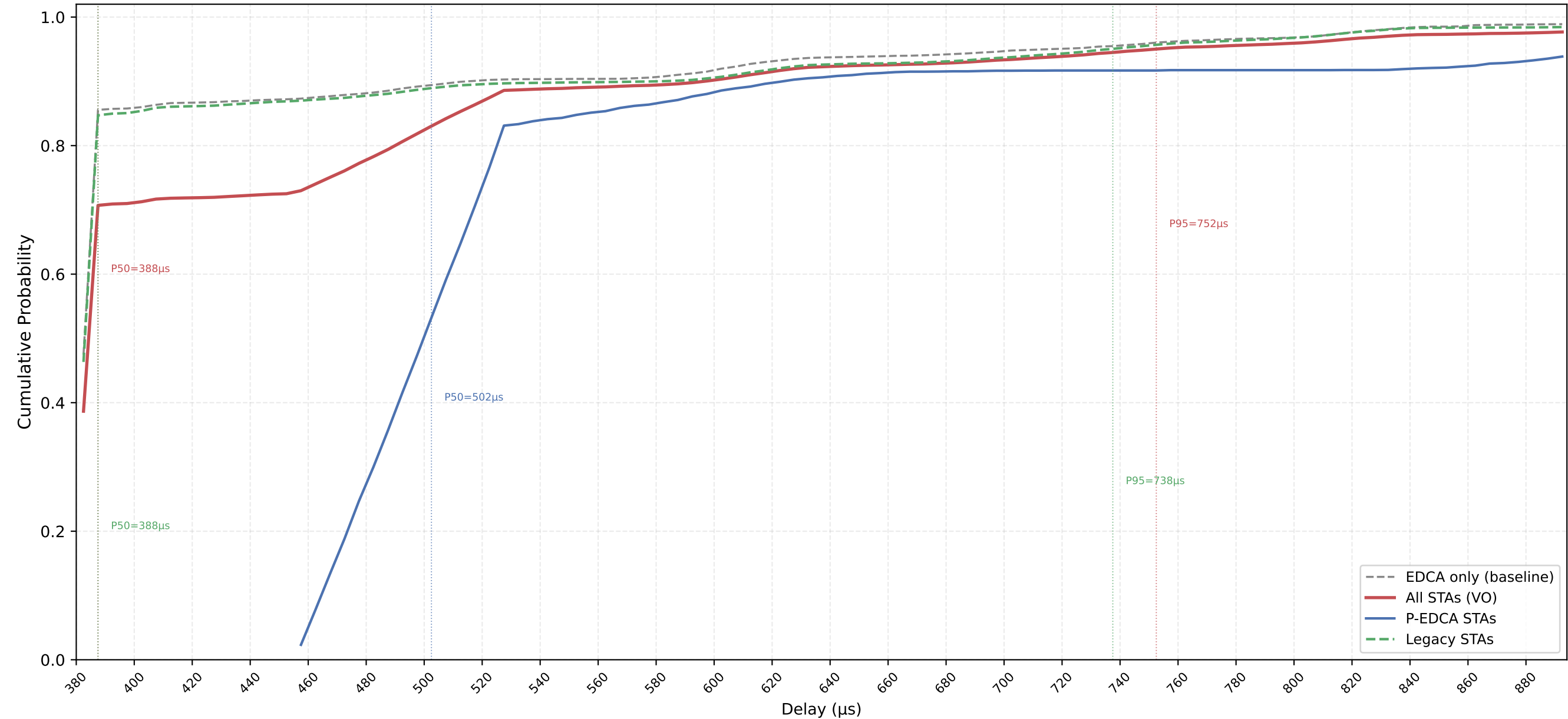
VO Delay CDF — P-EDCA / Legacy / All | CWds=1 × QSRC=0 × PSRC=1 nSta=30, nPedca=5/30, 0.1Mbps, avg of 10 runs
