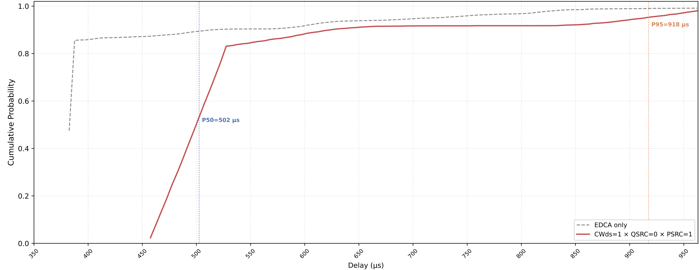
P-EDCA STA VO Delay CDF — CWds=1 × QSRC=0 × PSRC=1 nSta=30, nPedca=5, 0.1Mbps, avg of 10 runs
