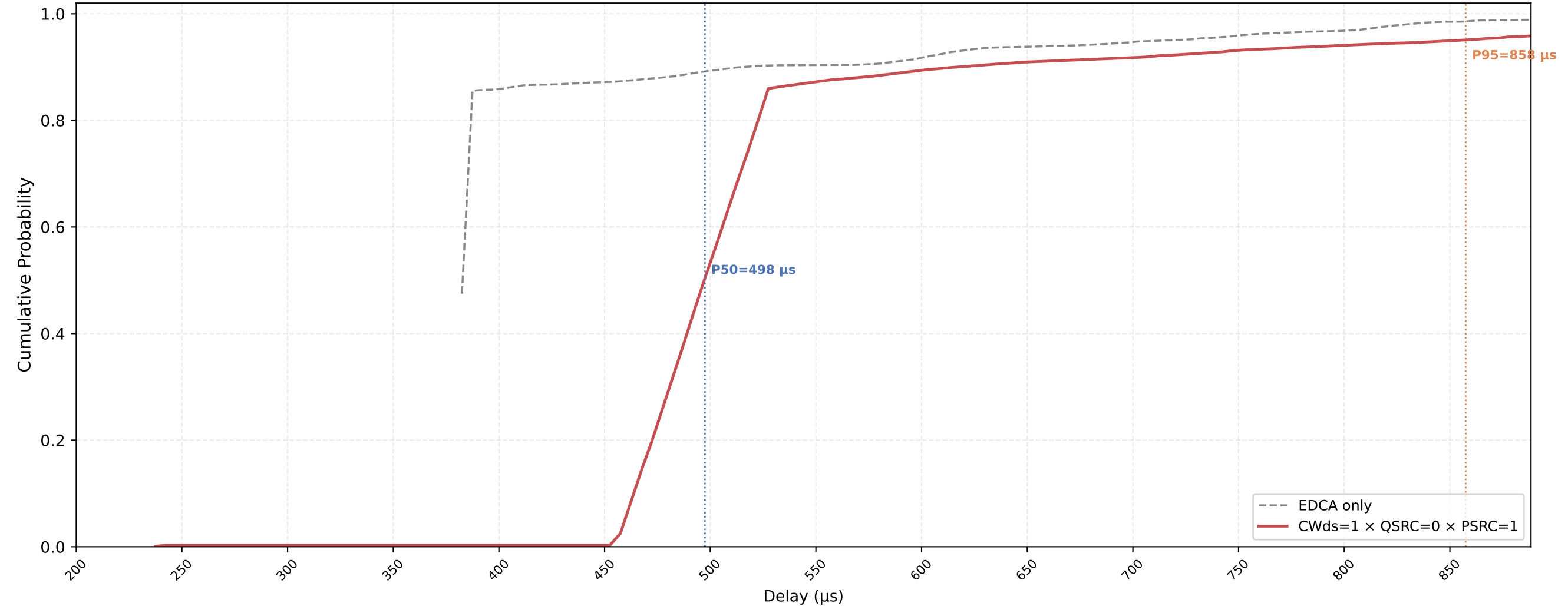
P-EDCA STA VO Delay CDF — CWds=1 × QSRC=0 × PSRC=1 nSta=30, nPedca=15, 0.1Mbps, avg of 10 runs
