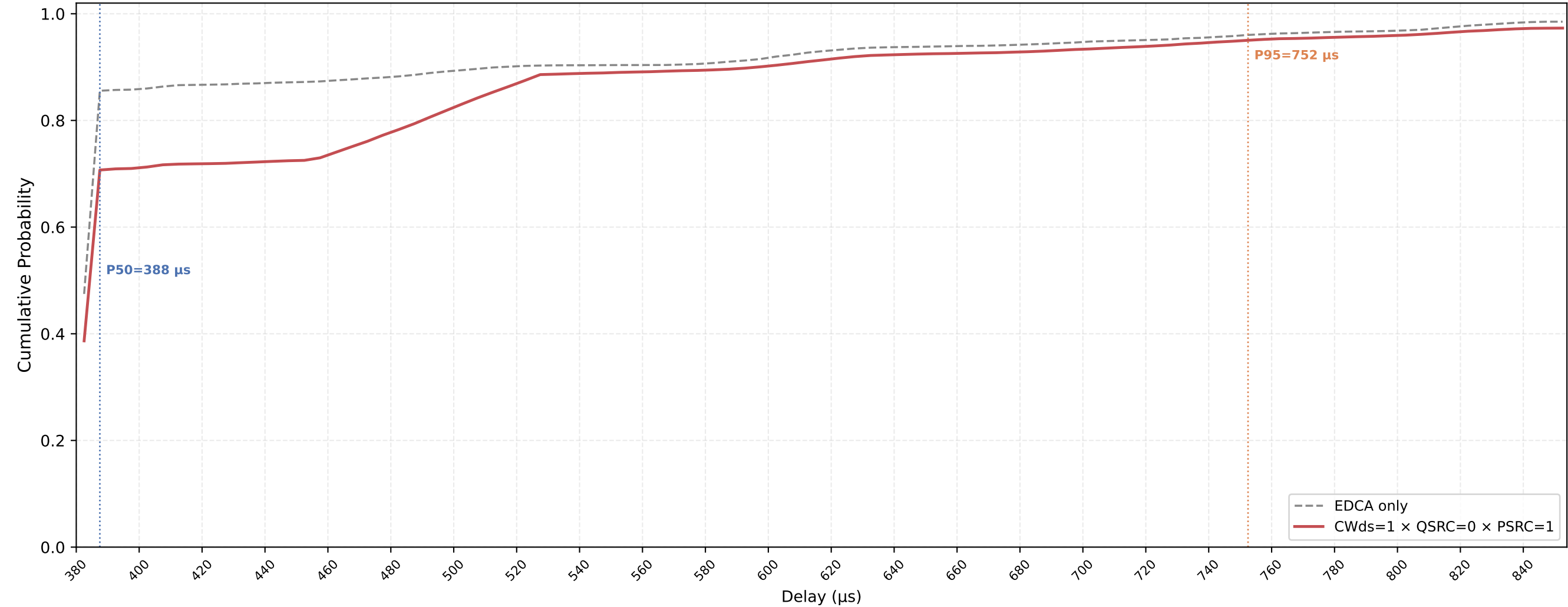
VO (all STAs) Delay CDF — CWds=1 × QSRC=0 × PSRC=1 nSta=30, nPedca=5, 0.1Mbps, avg of 10 runs
