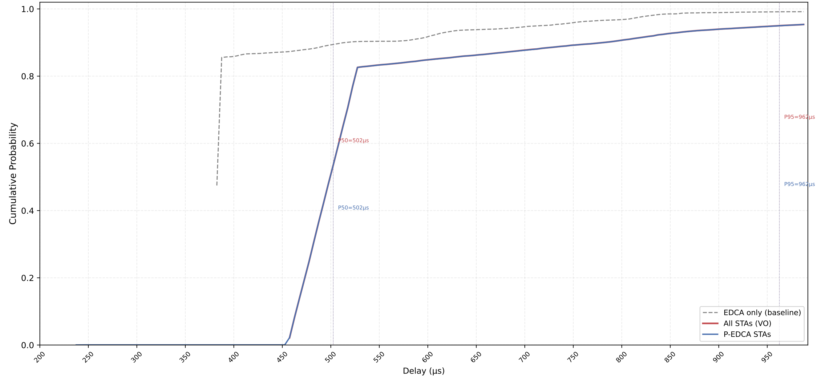
VO Delay CDF — P-EDCA / Legacy / All | CWds=1 × QSRC=0 × PSRC=2 nSta=30, nPedca=30/30, 0.1Mbps, avg of 10 runs
