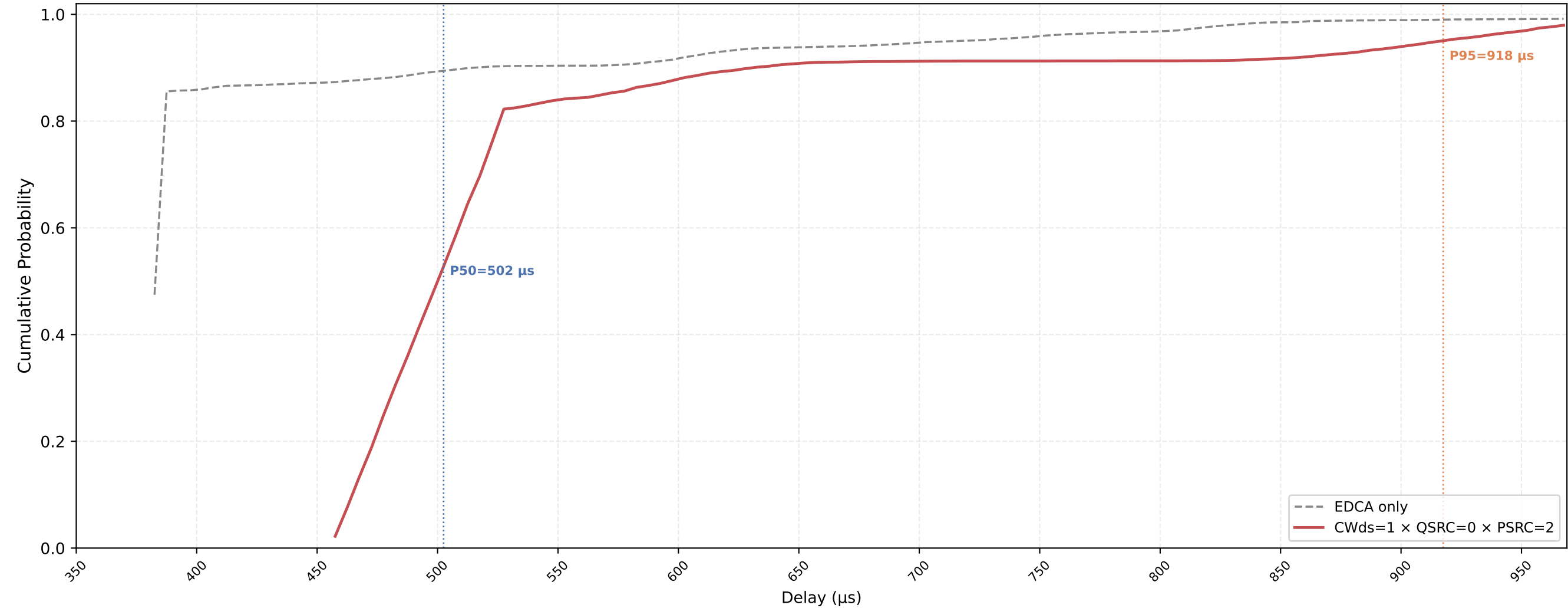
P-EDCA STA VO Delay CDF — CWds=1 × QSRC=0 × PSRC=2 nSta=30, nPedca=5, 0.1Mbps, avg of 10 runs
