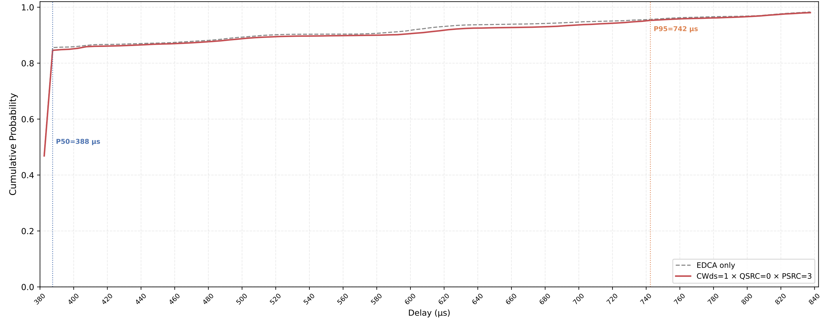
Legacy STA VO Delay CDF — CWds=1 × QSRC=0 × PSRC=3 nSta=30, nPedca=5, 0.1Mbps, avg of 10 runs
