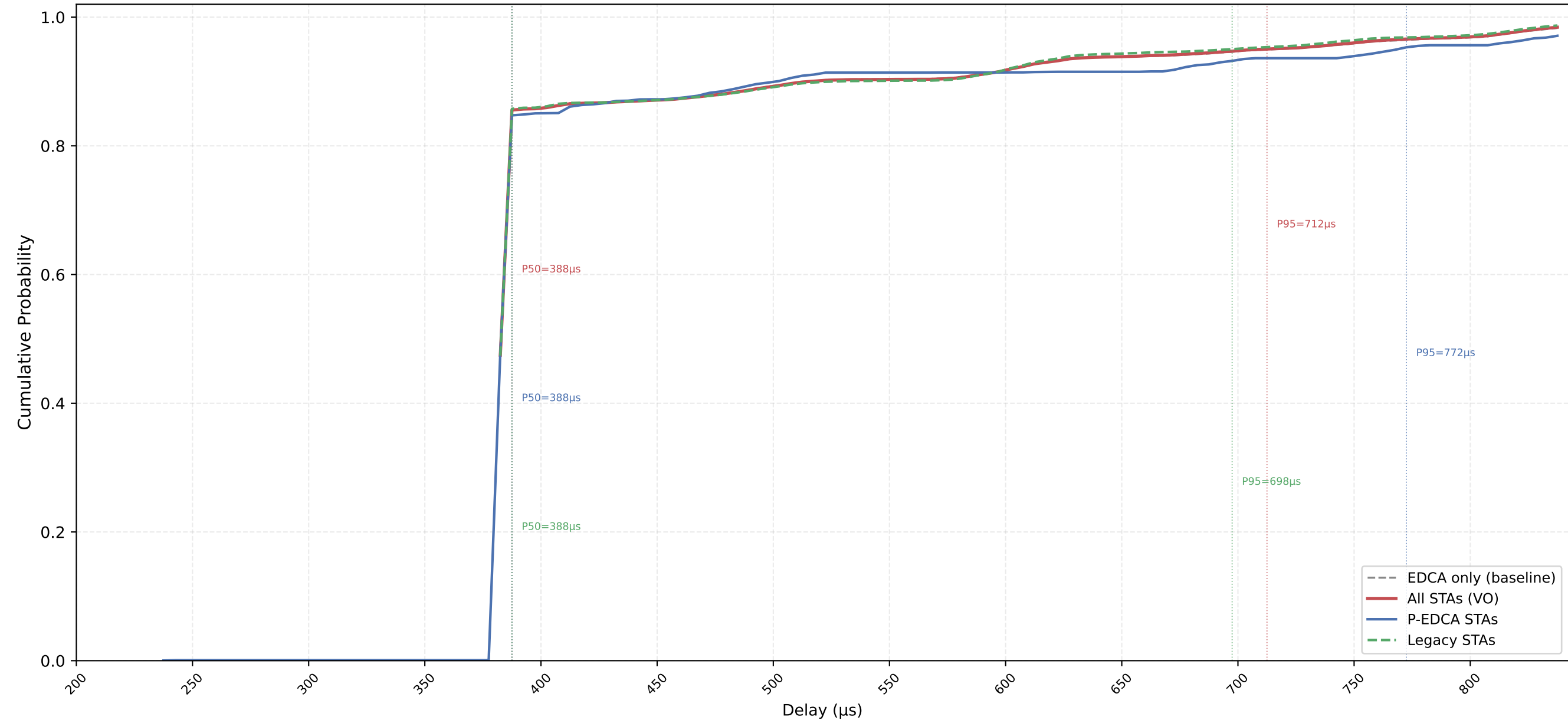
VO Delay CDF — P-EDCA / Legacy / All | CWds=1 × QSRC=1 × PSRC=1 nSta=30, nPedca=5/30, 0.1Mbps, avg of 10 runs
