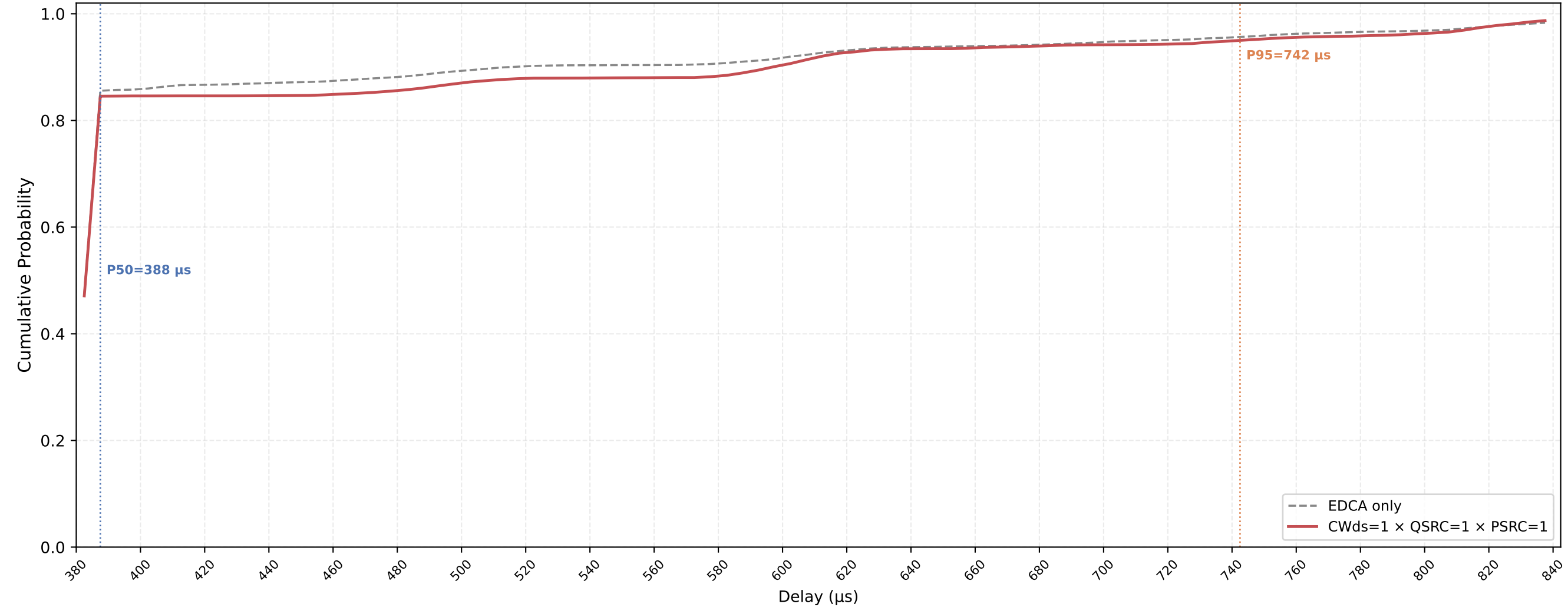
Legacy STA VO Delay CDF — CWds=1 × QSRC=1 × PSRC=1 nSta=30, nPedca=15, 0.1Mbps, avg of 10 runs
