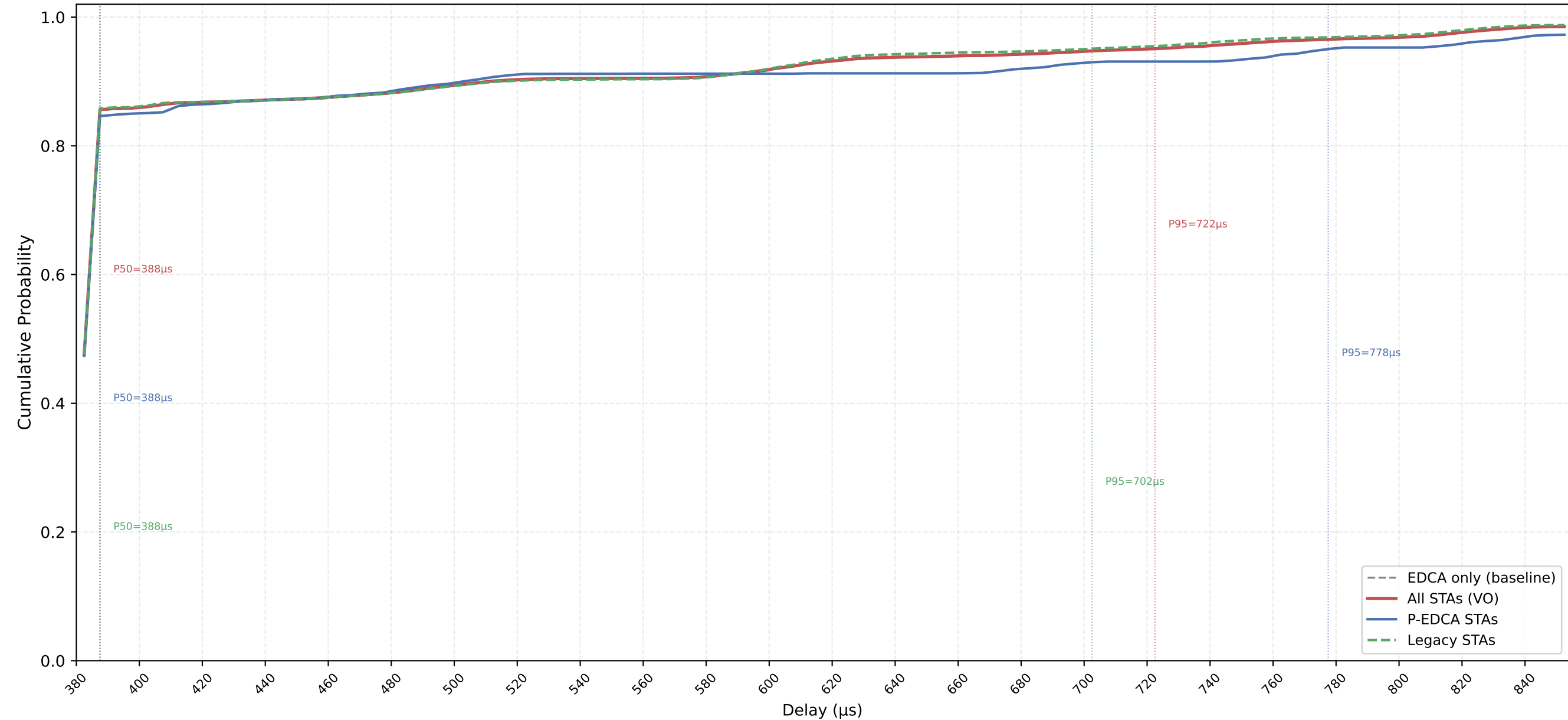
VO Delay CDF — P-EDCA / Legacy / All | CWds=1 × QSRC=1 × PSRC=2 nSta=30, nPedca=5/30, 0.1Mbps, avg of 10 runs
