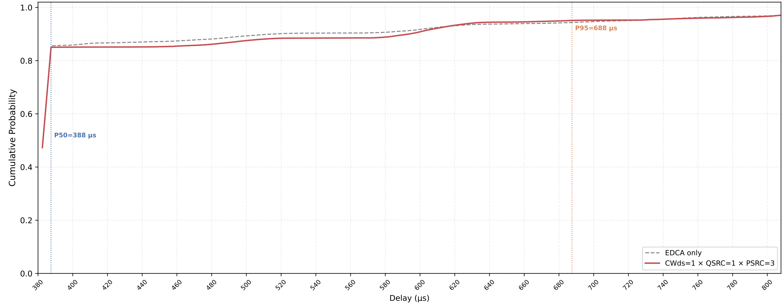
Legacy STA VO Delay CDF — CWds=1 × QSRC=1 × PSRC=3 nSta=30, nPedca=15, 0.1Mbps, avg of 10 runs
