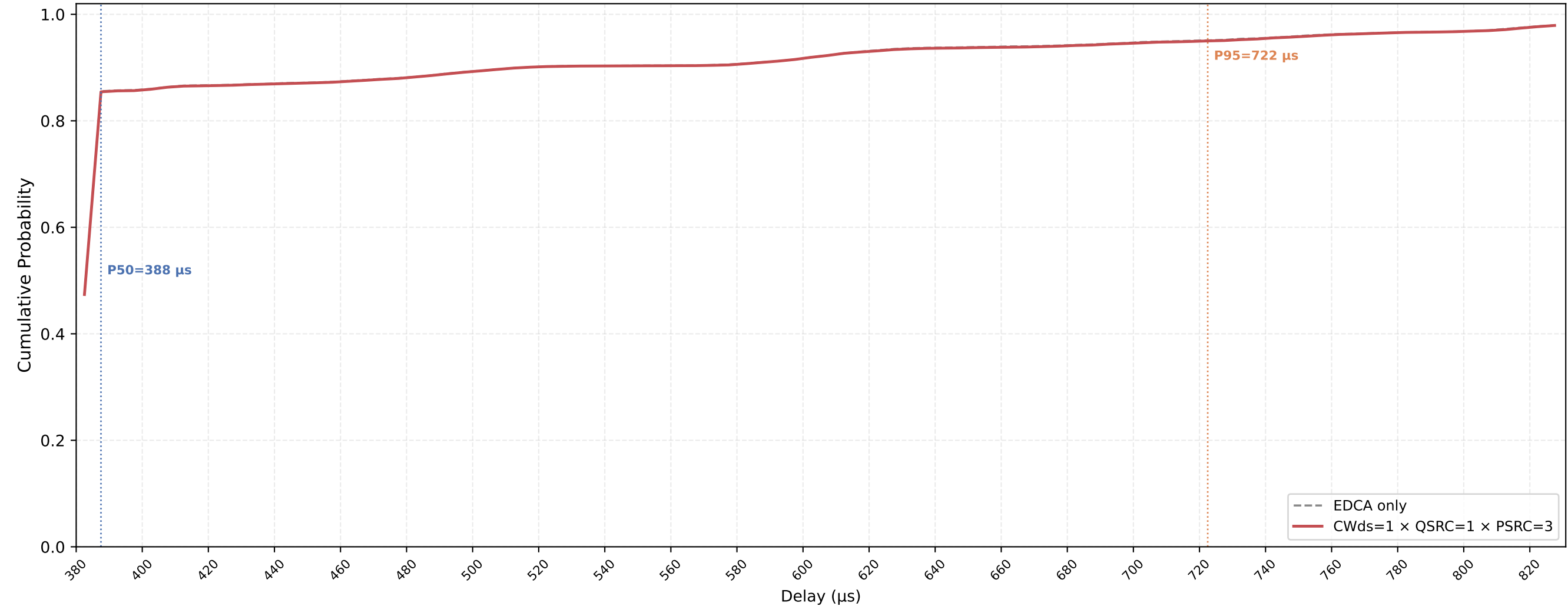
VO (all STAs) Delay CDF — CWds=1 × QSRC=1 × PSRC=3 nSta=30, nPedca=5, 0.1Mbps, avg of 10 runs
