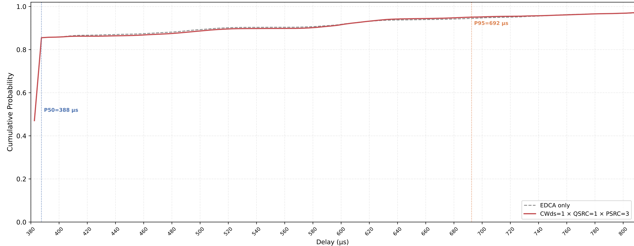
VO (all STAs) Delay CDF — CWds=1 × QSRC=1 × PSRC=3 nSta=30, nPedca=15, 0.1Mbps, avg of 10 runs
