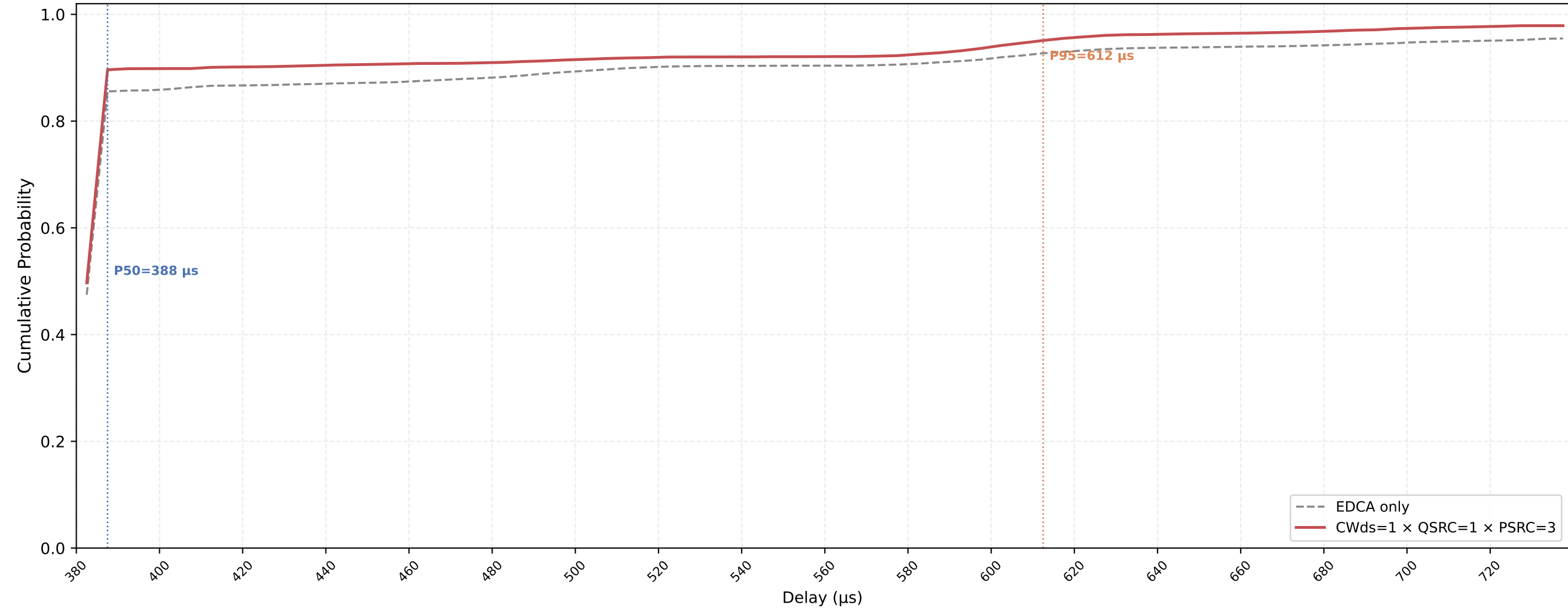
VO (all STAs) Delay CDF — CWds=1 × QSRC=1 × PSRC=3 nSta=30, nPedca=30, 0.1Mbps, avg of 10 runs
