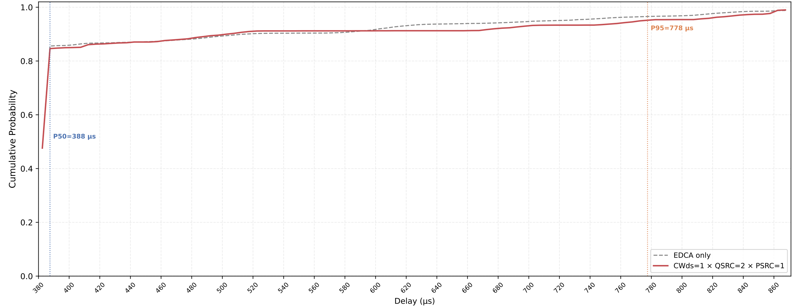
P-EDCA STA VO Delay CDF — CWds=1 × QSRC=2 × PSRC=1 nSta=30, nPedca=5, 0.1Mbps, avg of 10 runs
