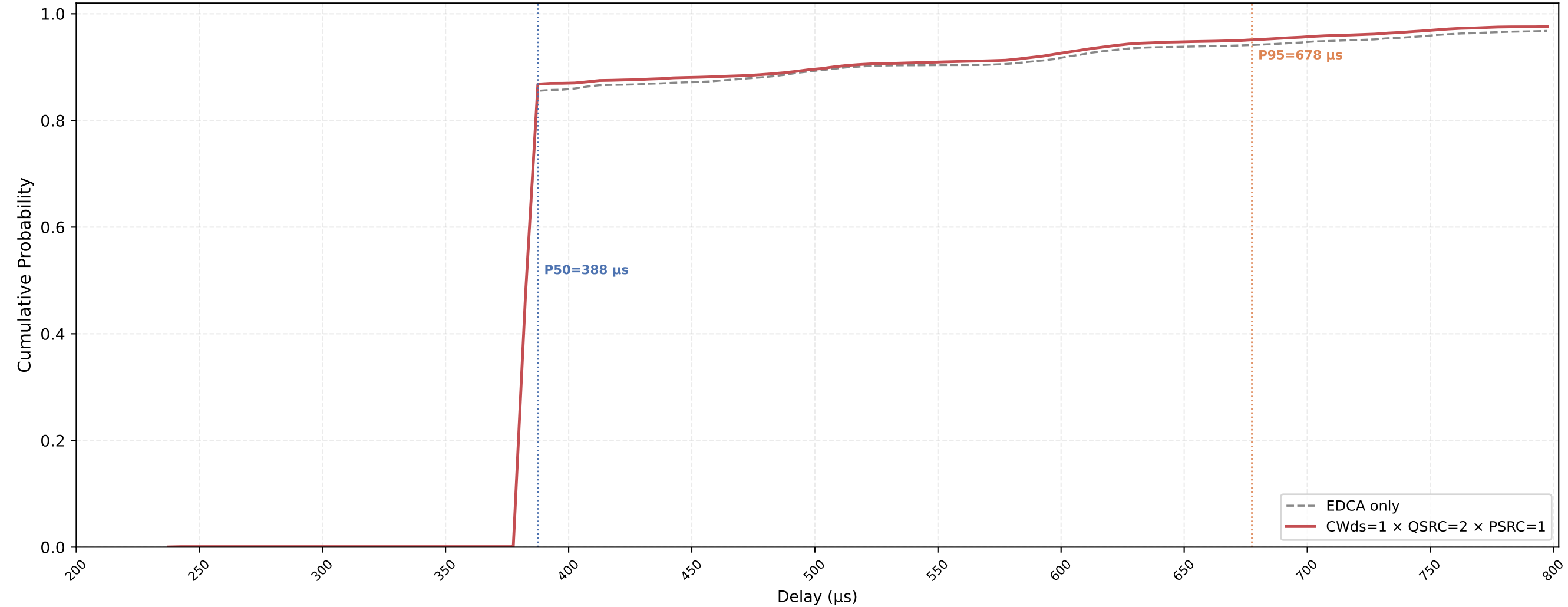
P-EDCA STA VO Delay CDF — CWds=1 × QSRC=2 × PSRC=1 nSta=30, nPedca=30, 0.1Mbps, avg of 10 runs
