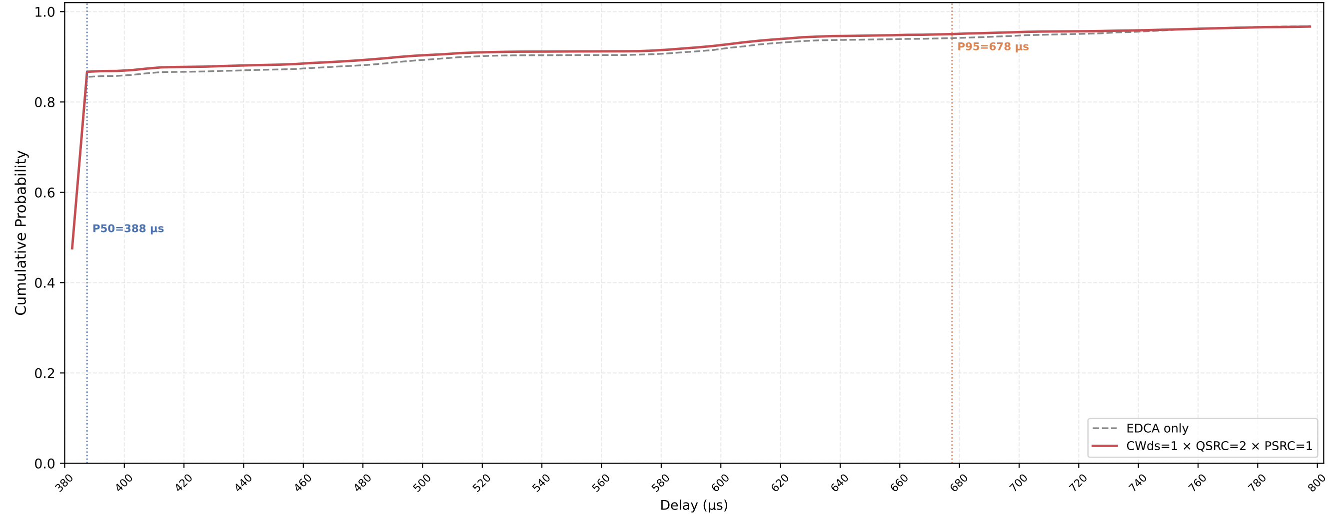
VO (all STAs) Delay CDF — CWds=1 × QSRC=2 × PSRC=1 nSta=30, nPedca=15, 0.1Mbps, avg of 10 runs
