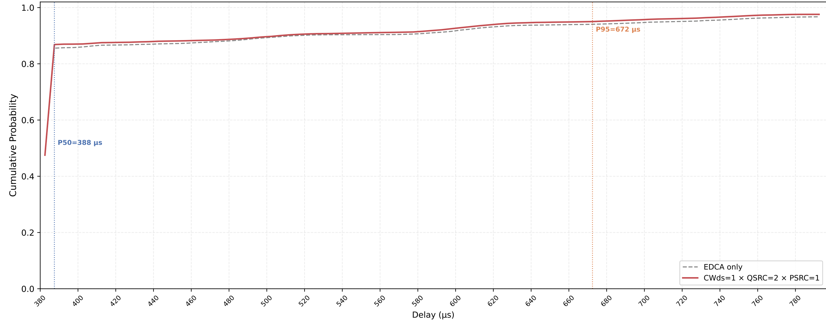
VO (all STAs) Delay CDF — CWds=1 × QSRC=2 × PSRC=1 nSta=30, nPedca=30, 0.1Mbps, avg of 10 runs
