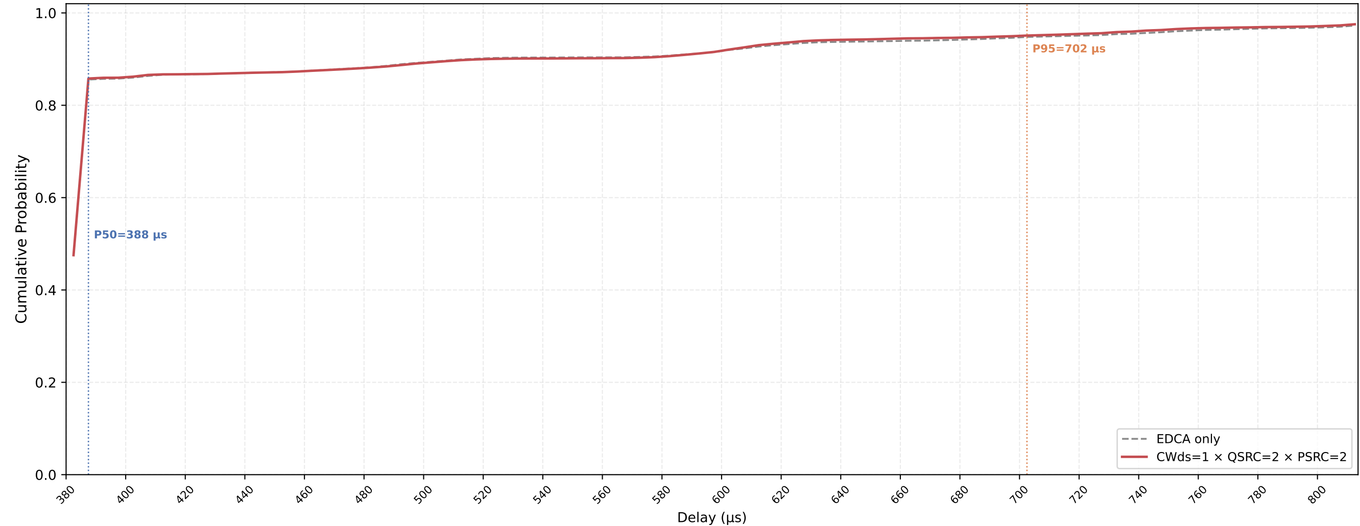
Legacy STA VO Delay CDF — CWds=1 × QSRC=2 × PSRC=2 nSta=30, nPedca=5, 0.1Mbps, avg of 10 runs
