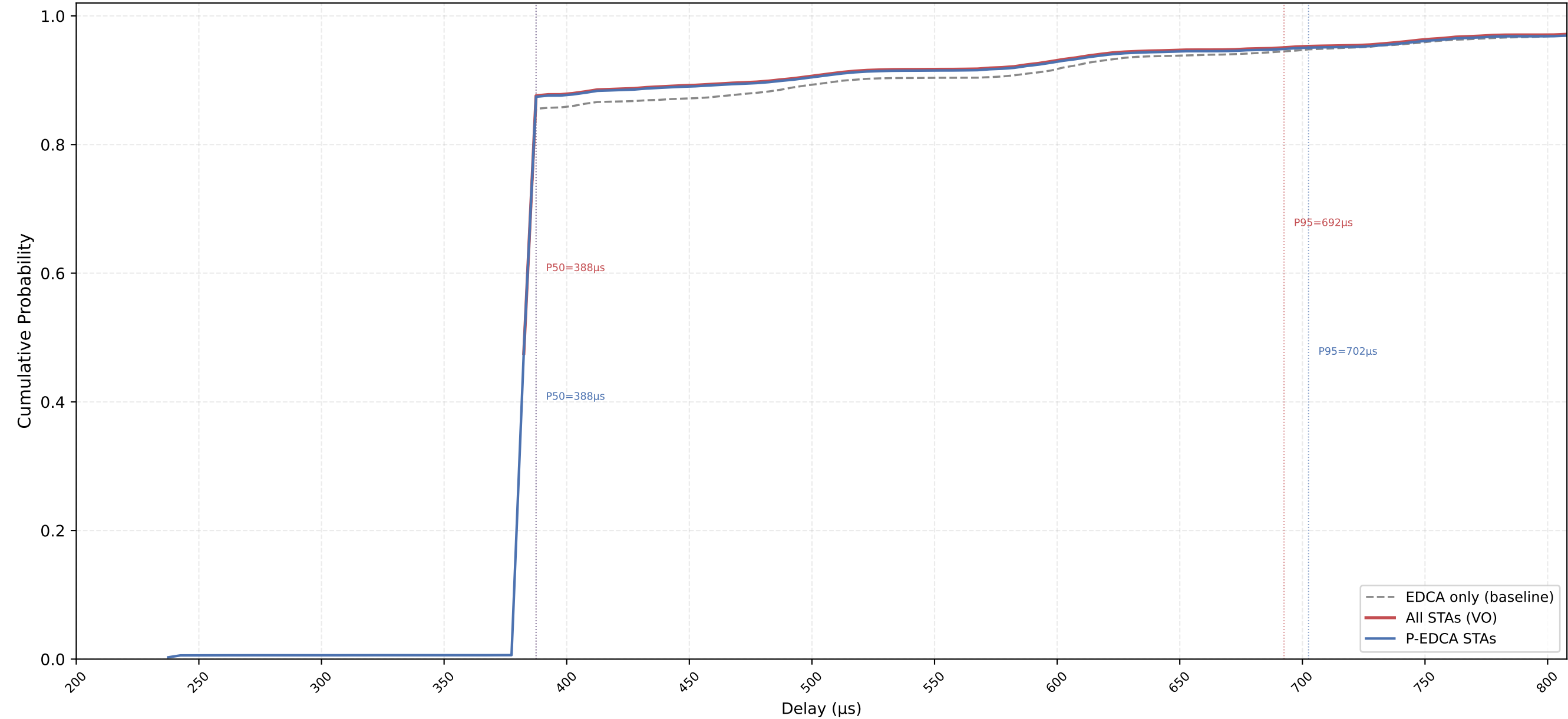
VO Delay CDF — P-EDCA / Legacy / All | CWds=1 × QSRC=2 × PSRC=3 nSta=30, nPedca=30/30, 0.1Mbps, avg of 10 runs
