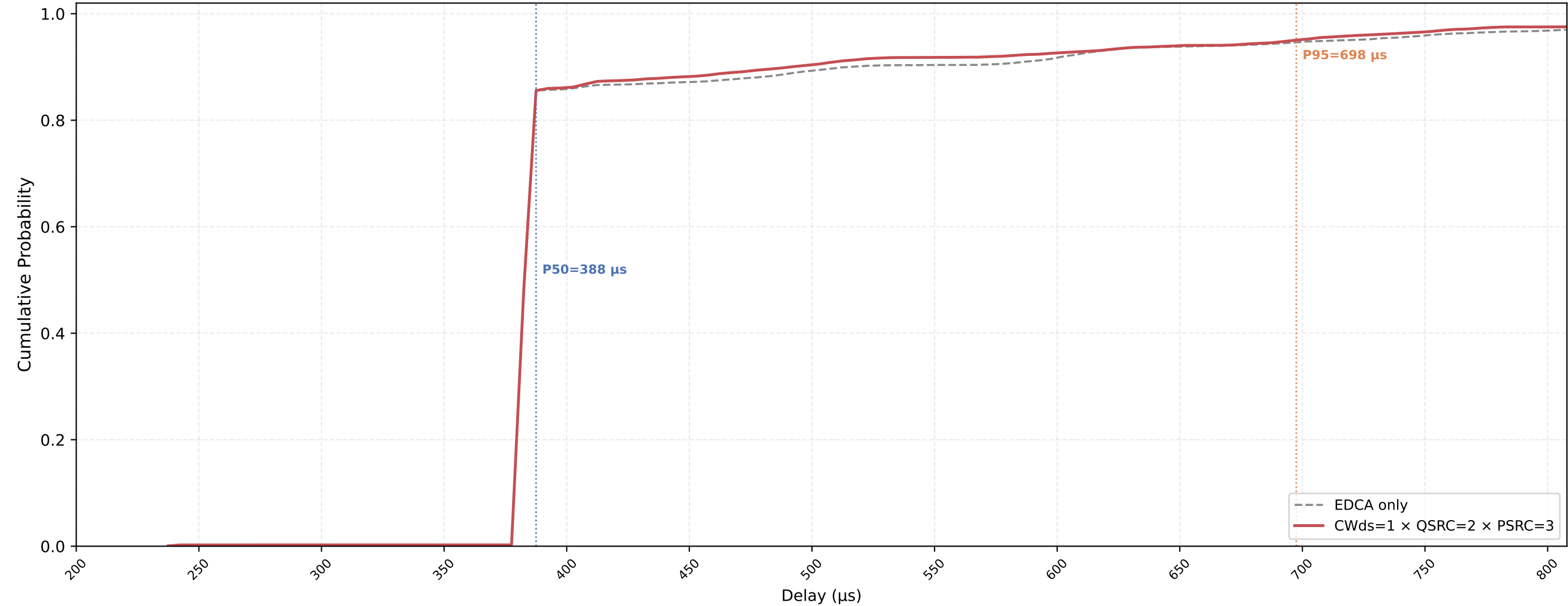
P-EDCA STA VO Delay CDF — CWds=1 × QSRC=2 × PSRC=3 nSta=30, nPedca=15, 0.1Mbps, avg of 10 runs
