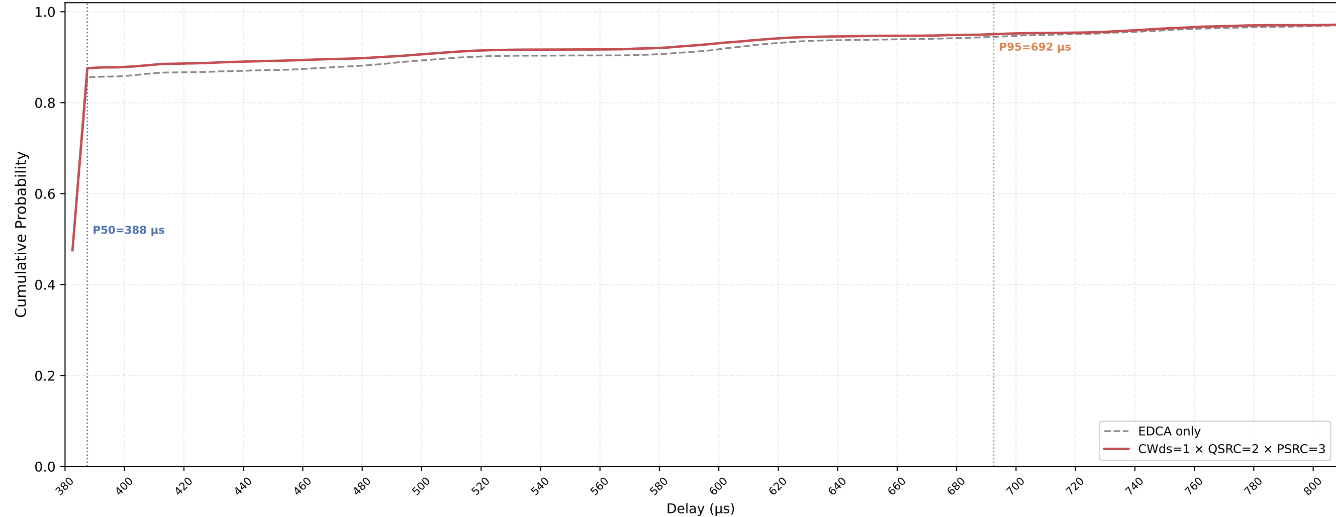
VO (all STAs) Delay CDF — CWds=1 × QSRC=2 × PSRC=3 nSta=30, nPedca=30, 0.1Mbps, avg of 10 runs
