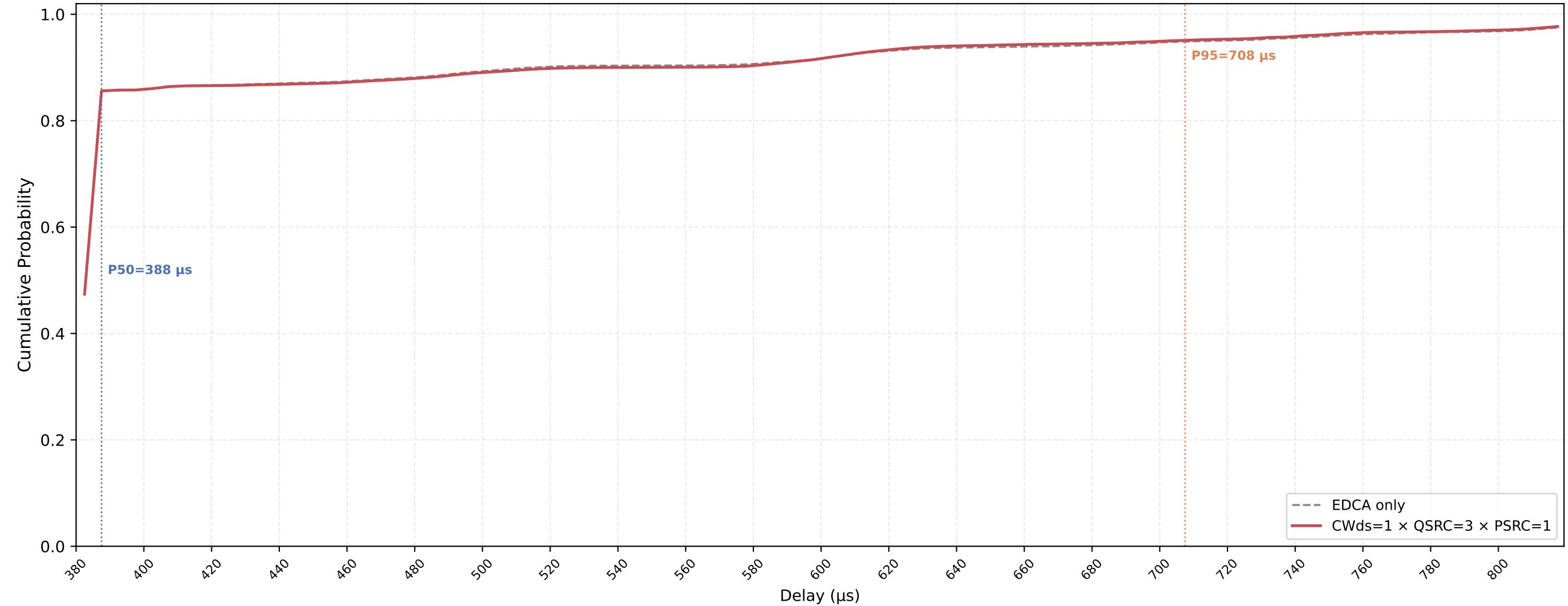
Legacy STA VO Delay CDF — CWds=1 × QSRC=3 × PSRC=1 nSta=30, nPedca=5, 0.1Mbps, avg of 10 runs
