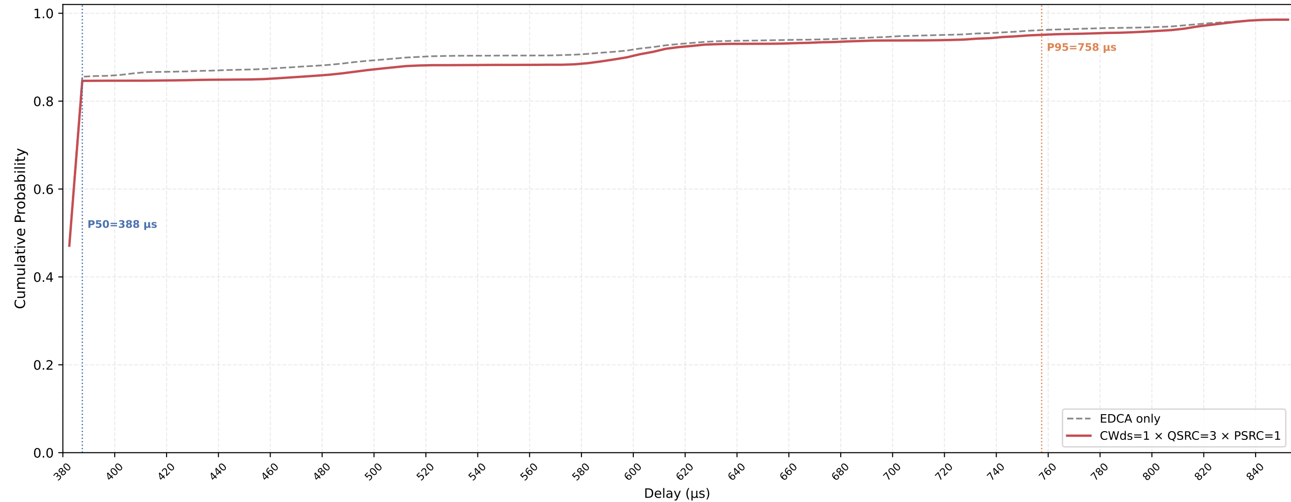
Legacy STA VO Delay CDF — CWds=1 × QSRC=3 × PSRC=1 nSta=30, nPedca=15, 0.1Mbps, avg of 10 runs
