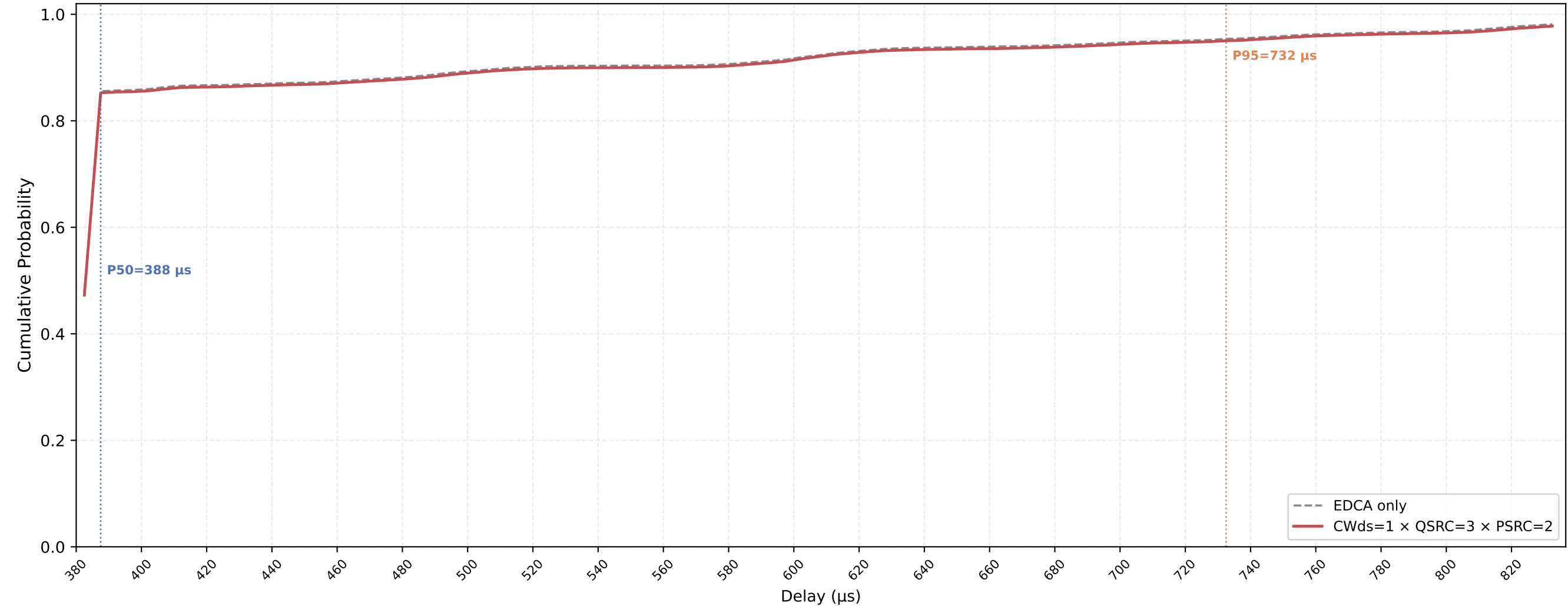
VO (all STAs) Delay CDF — CWds=1 × QSRC=3 × PSRC=2 nSta=30, nPedca=30, 0.1Mbps, avg of 10 runs
