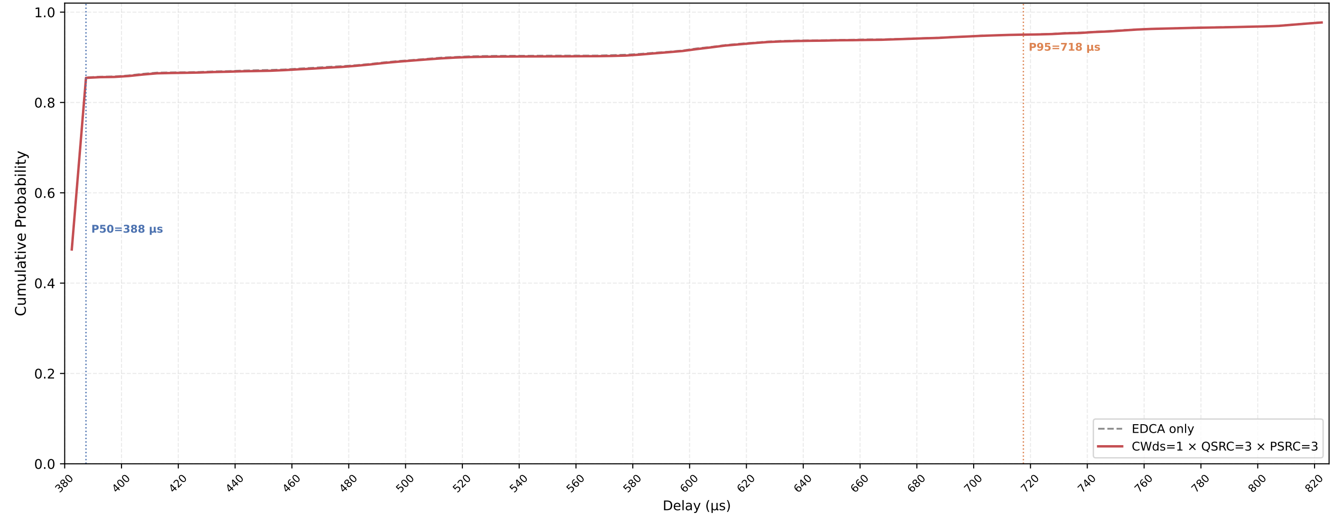
VO (all STAs) Delay CDF — CWds=1 × QSRC=3 × PSRC=3 nSta=30, nPedca=5, 0.1Mbps, avg of 10 runs
