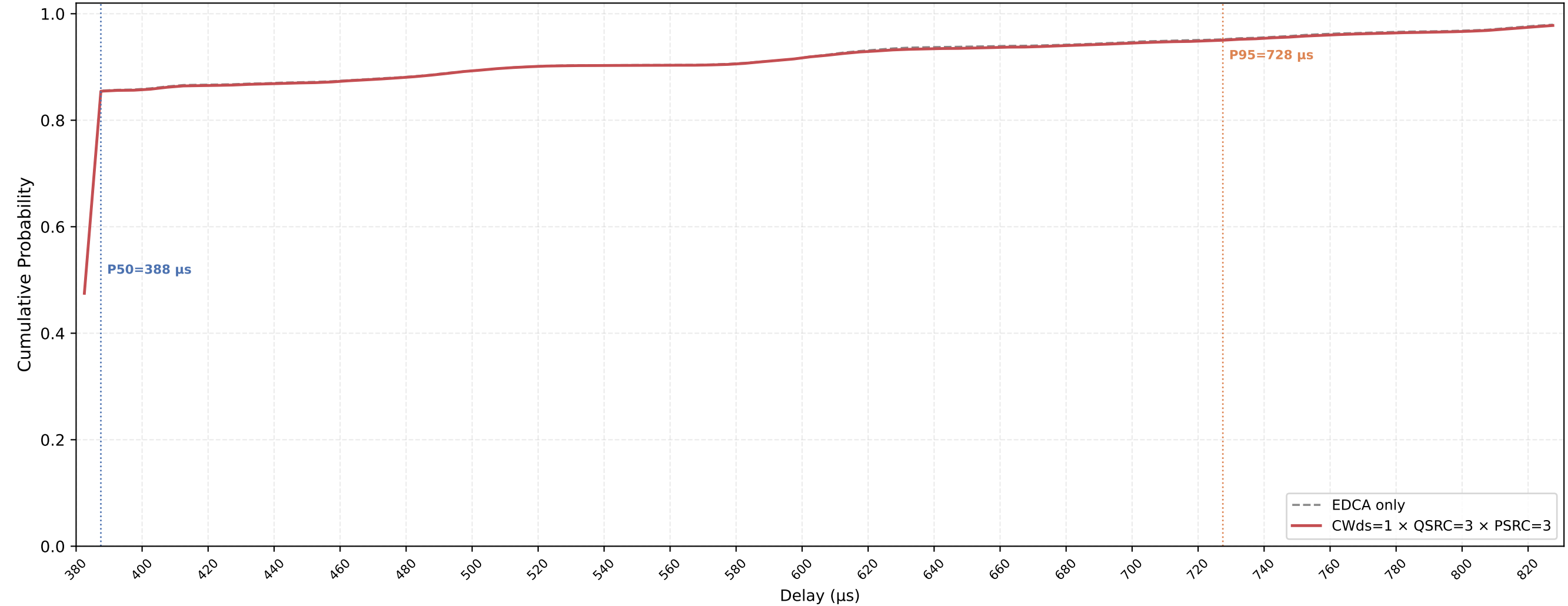
VO (all STAs) Delay CDF — CWds=1 × QSRC=3 × PSRC=3 nSta=30, nPedca=15, 0.1Mbps, avg of 10 runs
