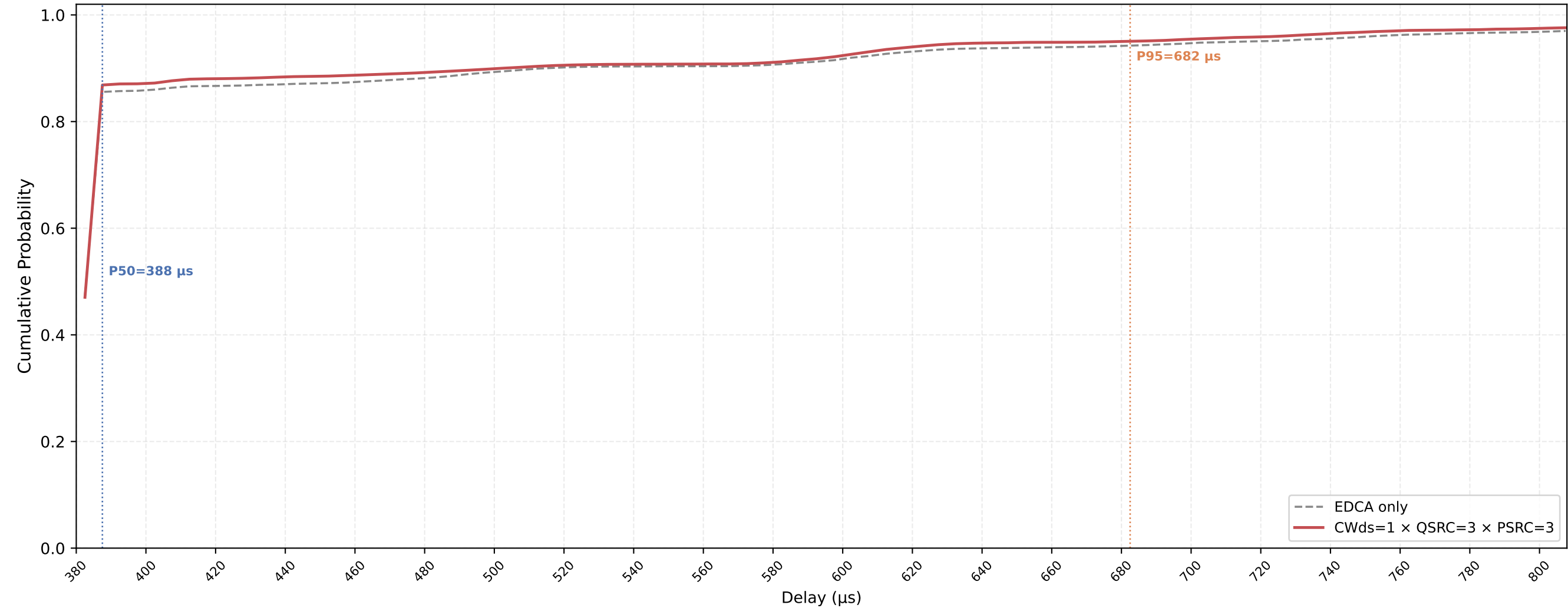
VO (all STAs) Delay CDF — CWds=1 × QSRC=3 × PSRC=3 nSta=30, nPedca=30, 0.1Mbps, avg of 10 runs
