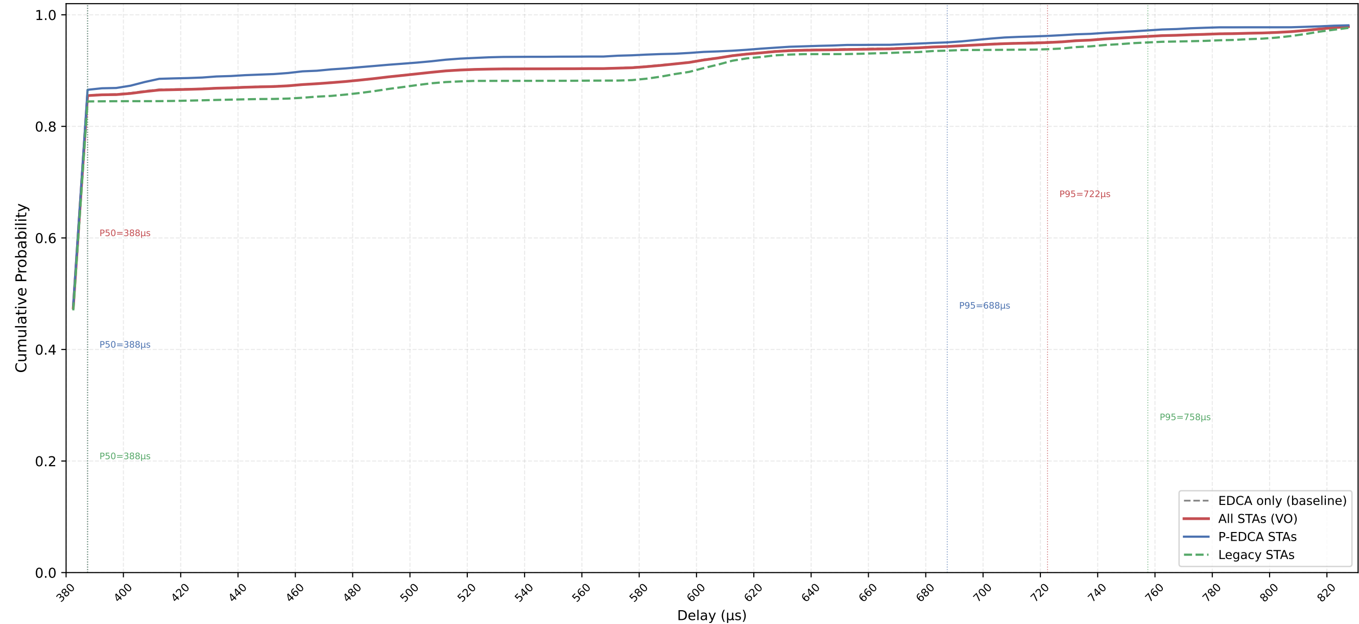
VO Delay CDF — P-EDCA / Legacy / All | CWds=1 × QSRC=4 × PSRC=1 nSta=30, nPedca=15/30, 0.1Mbps, avg of 10 runs
