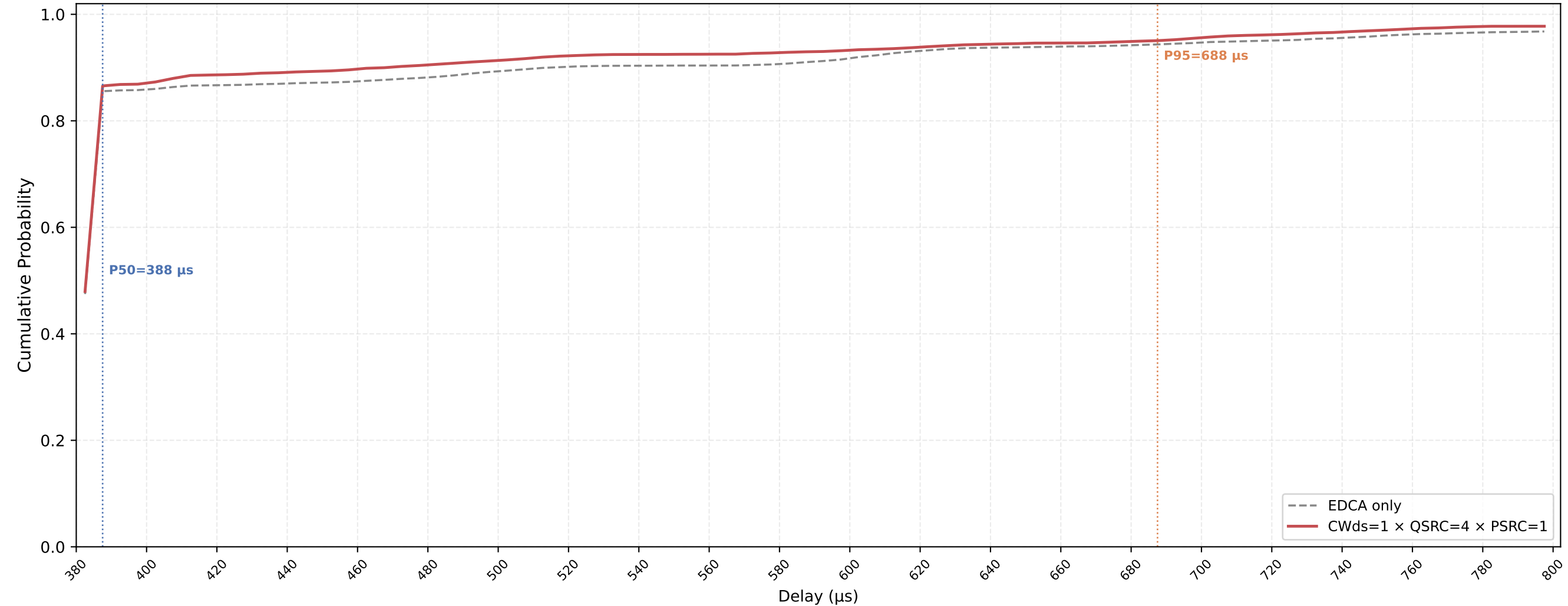
P-EDCA STA VO Delay CDF — CWds=1 × QSRC=4 × PSRC=1 nSta=30, nPedca=15, 0.1Mbps, avg of 10 runs
