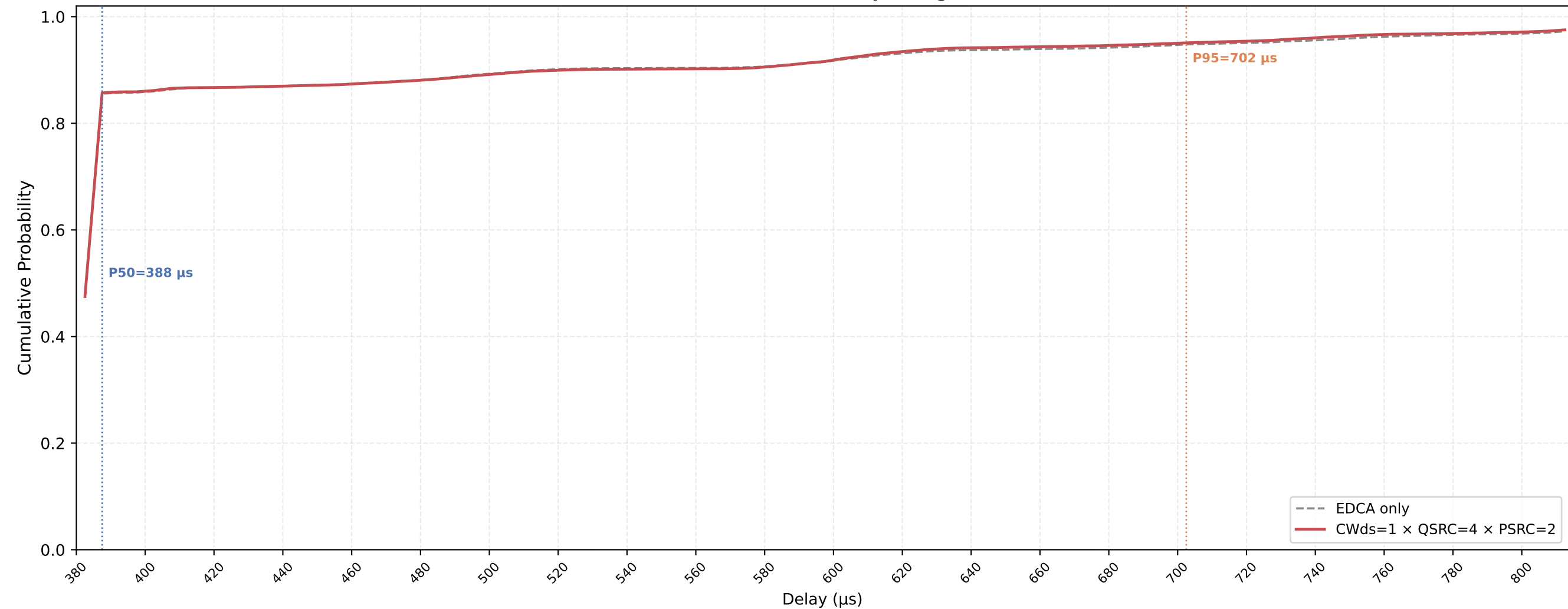
Legacy STA VO Delay CDF — CWds=1 × QSRC=4 × PSRC=2 nSta=30, nPedca=5, 0.1Mbps, avg of 10 runs
