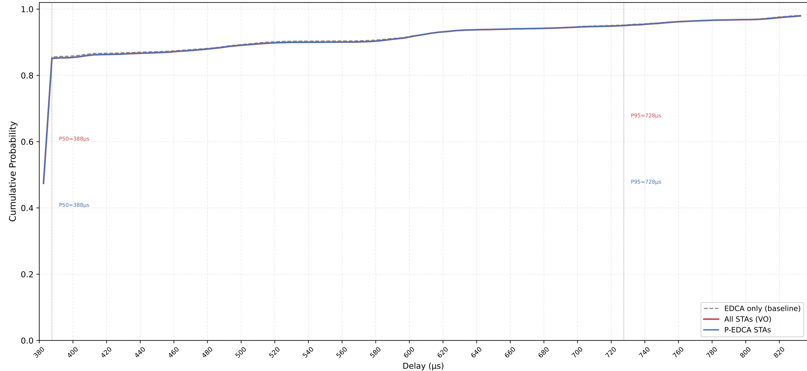
VO Delay CDF — P-EDCA / Legacy / All | CWds=1 × QSRC=5 × PSRC=1 nSta=30, nPedca=30/30, 0.1Mbps, avg of 10 runs
