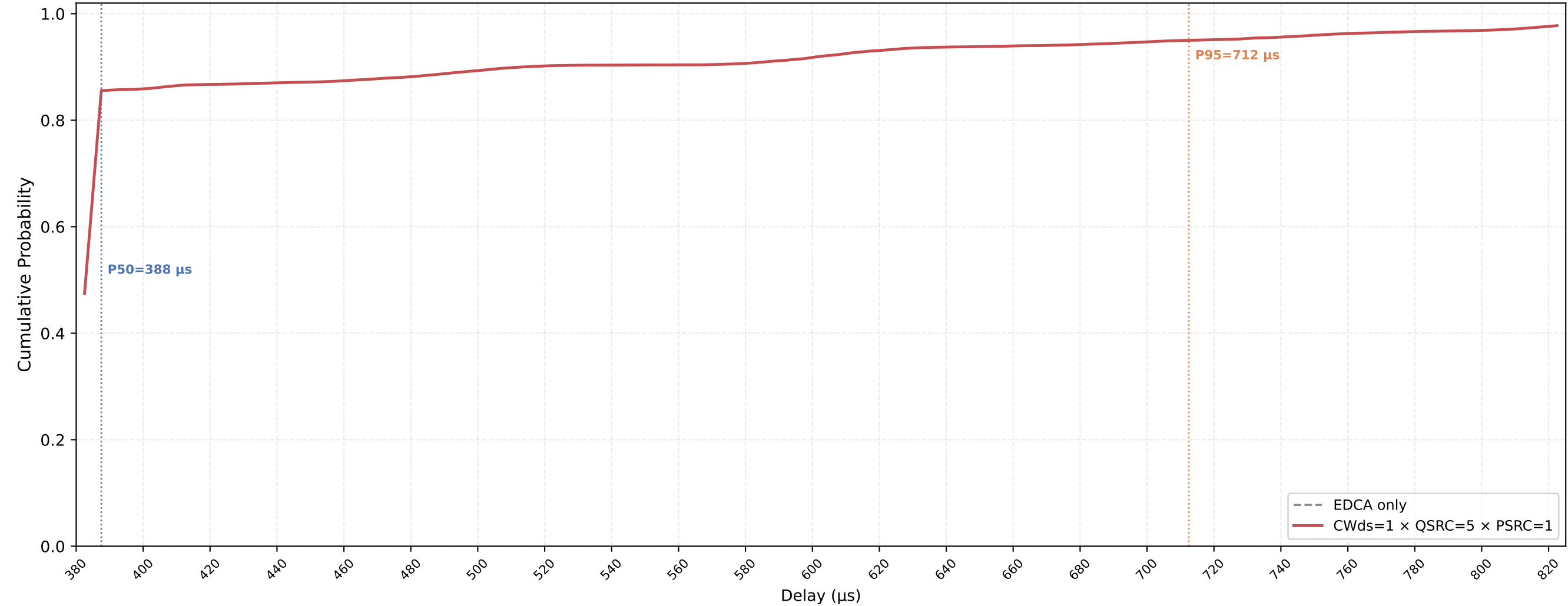
VO (all STAs) Delay CDF — CWds=1 × QSRC=5 × PSRC=1 nSta=30, nPedca=5, 0.1Mbps, avg of 10 runs
