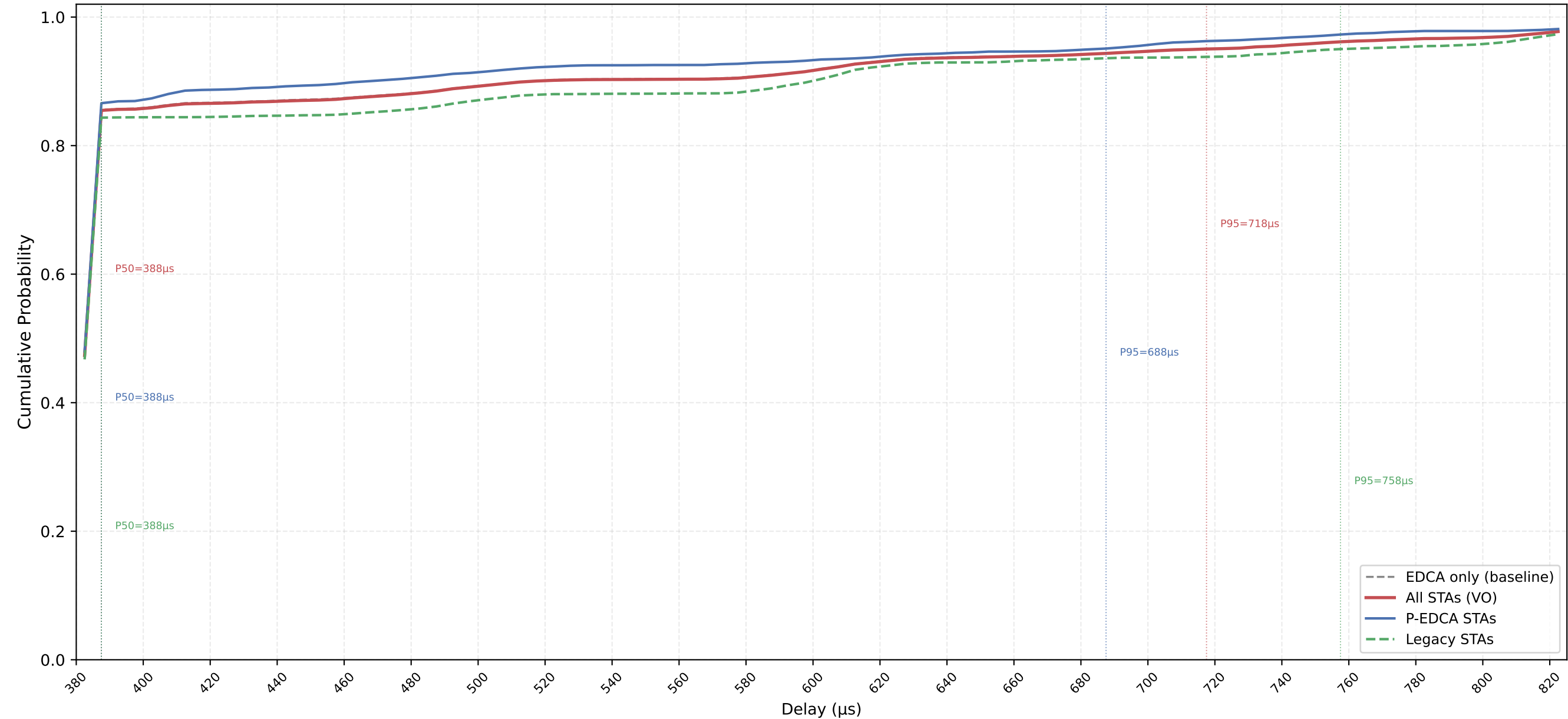
VO Delay CDF — P-EDCA / Legacy / All | CWds=1 × QSRC=5 × PSRC=2 nSta=30, nPedca=15/30, 0.1Mbps, avg of 10 runs
