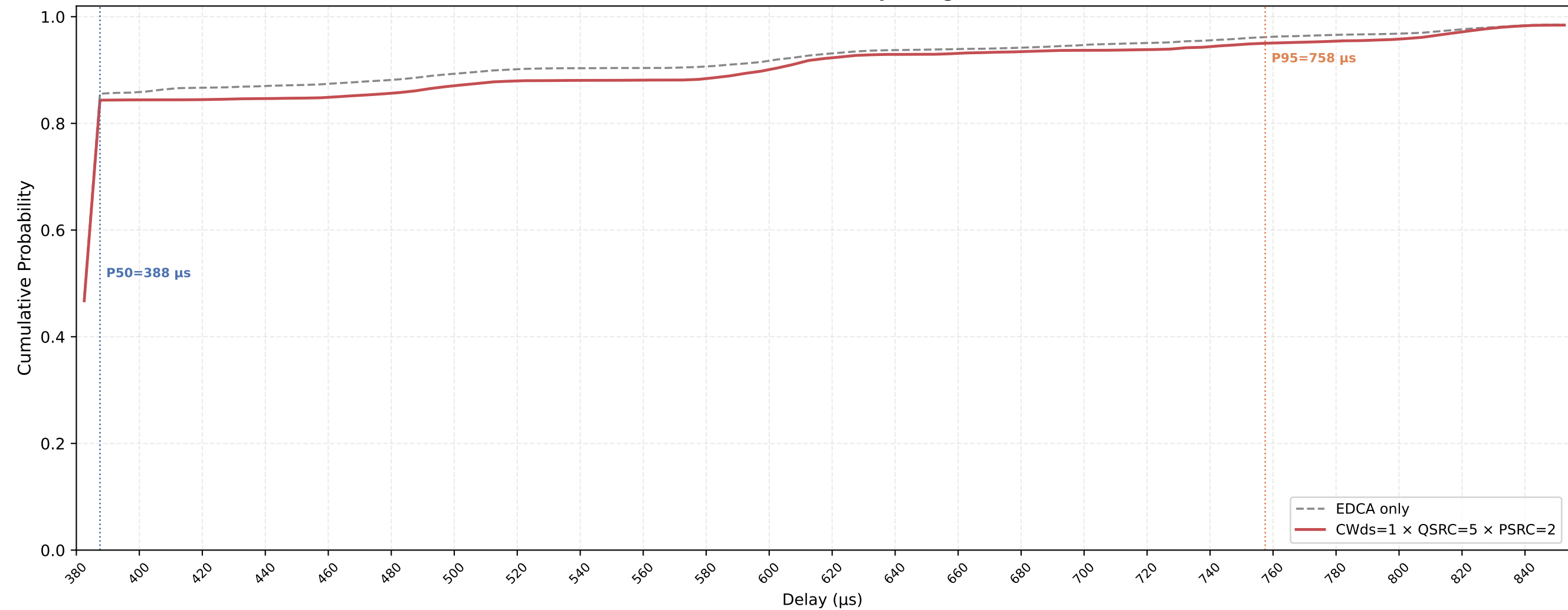
Legacy STA VO Delay CDF — CWds=1 × QSRC=5 × PSRC=2 nSta=30, nPedca=15, 0.1Mbps, avg of 10 runs
