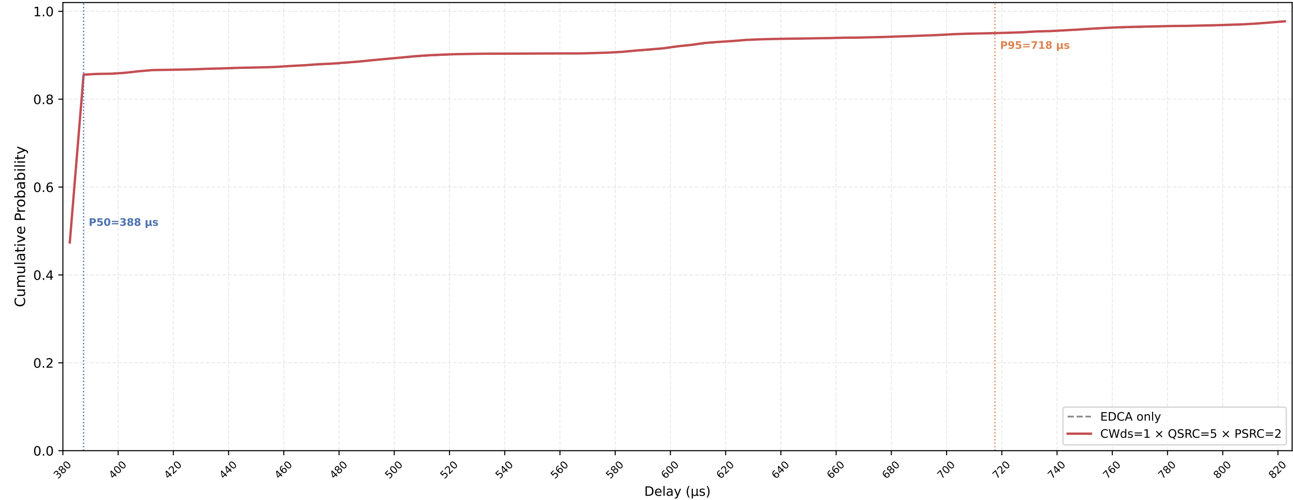
VO (all STAs) Delay CDF — CWds=1 × QSRC=5 × PSRC=2 nSta=30, nPedca=5, 0.1Mbps, avg of 10 runs
