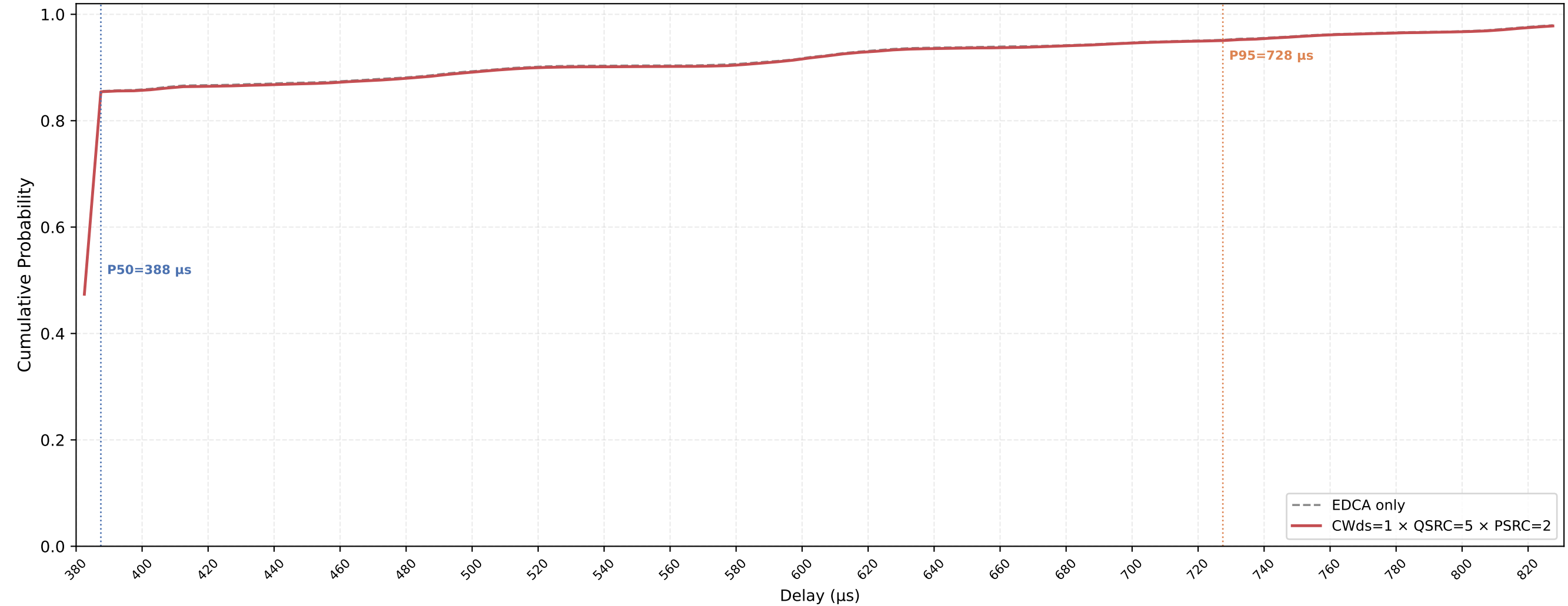
VO (all STAs) Delay CDF — CWds=1 × QSRC=5 × PSRC=2 nSta=30, nPedca=30, 0.1Mbps, avg of 10 runs
