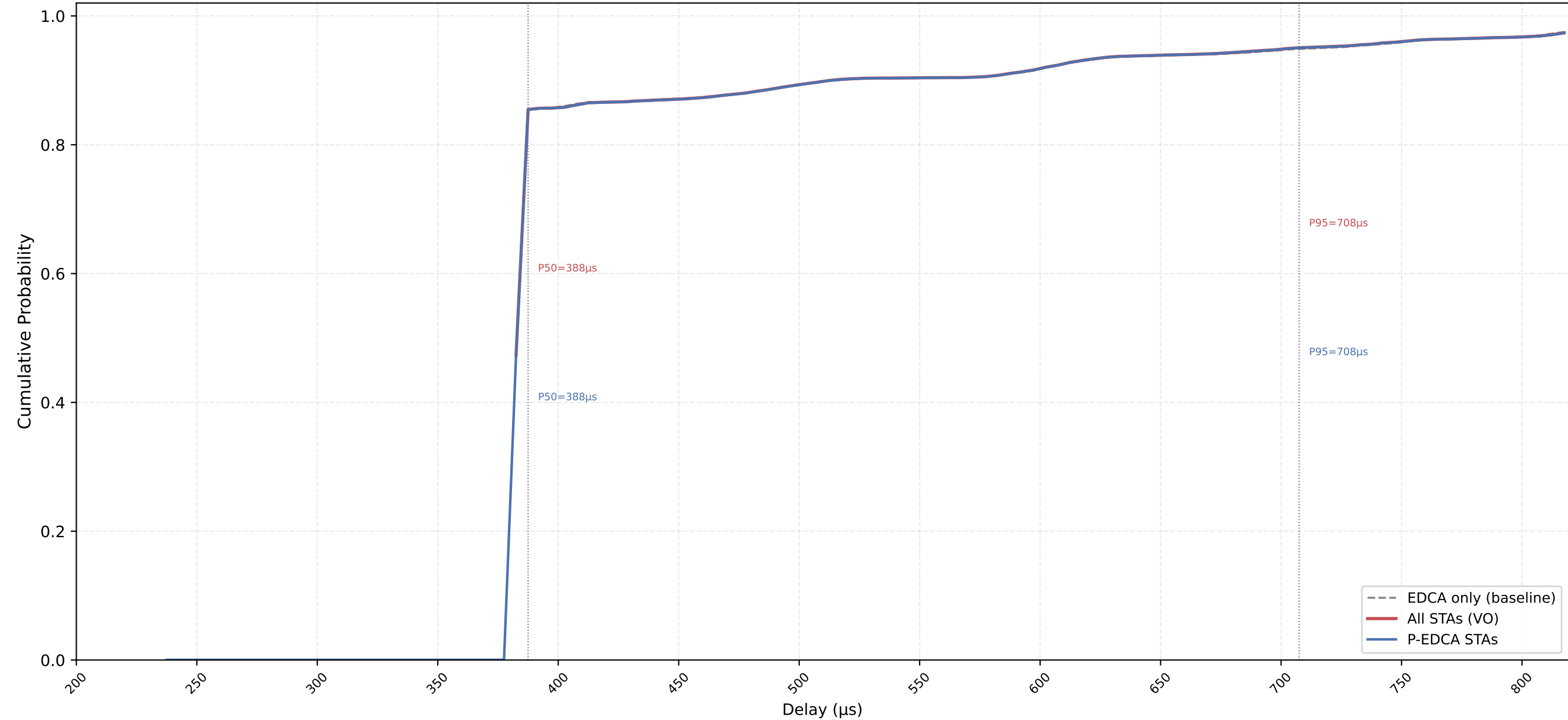
VO Delay CDF — P-EDCA / Legacy / All | CWds=1 × QSRC=5 × PSRC=3 nSta=30, nPedca=30/30, 0.1Mbps, avg of 10 runs
