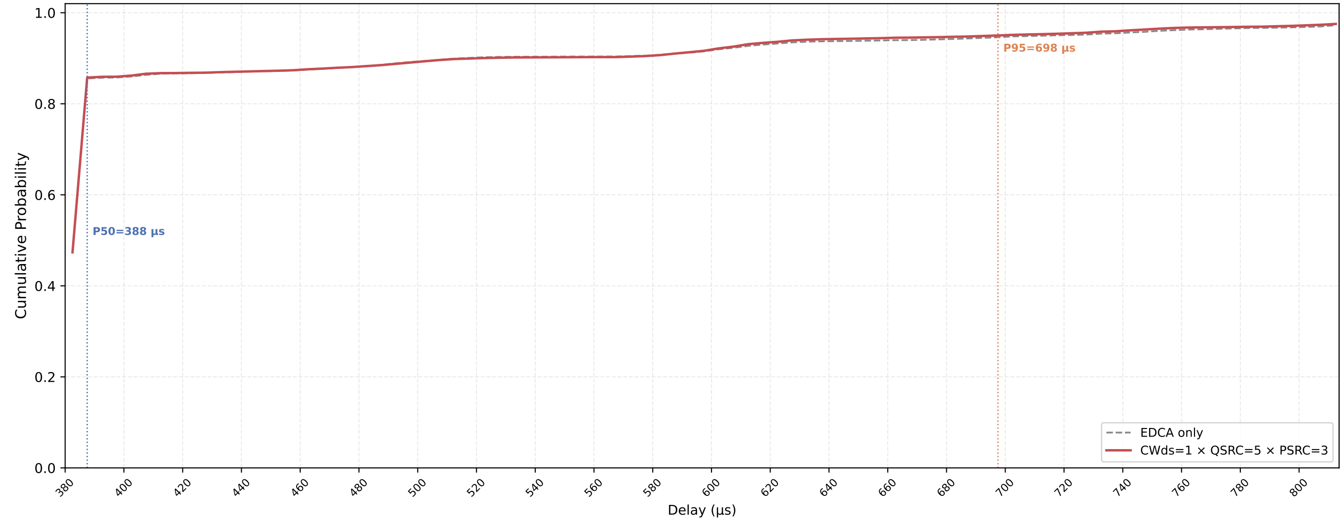
Legacy STA VO Delay CDF — CWds=1 × QSRC=5 × PSRC=3 nSta=30, nPedca=5, 0.1Mbps, avg of 10 runs
