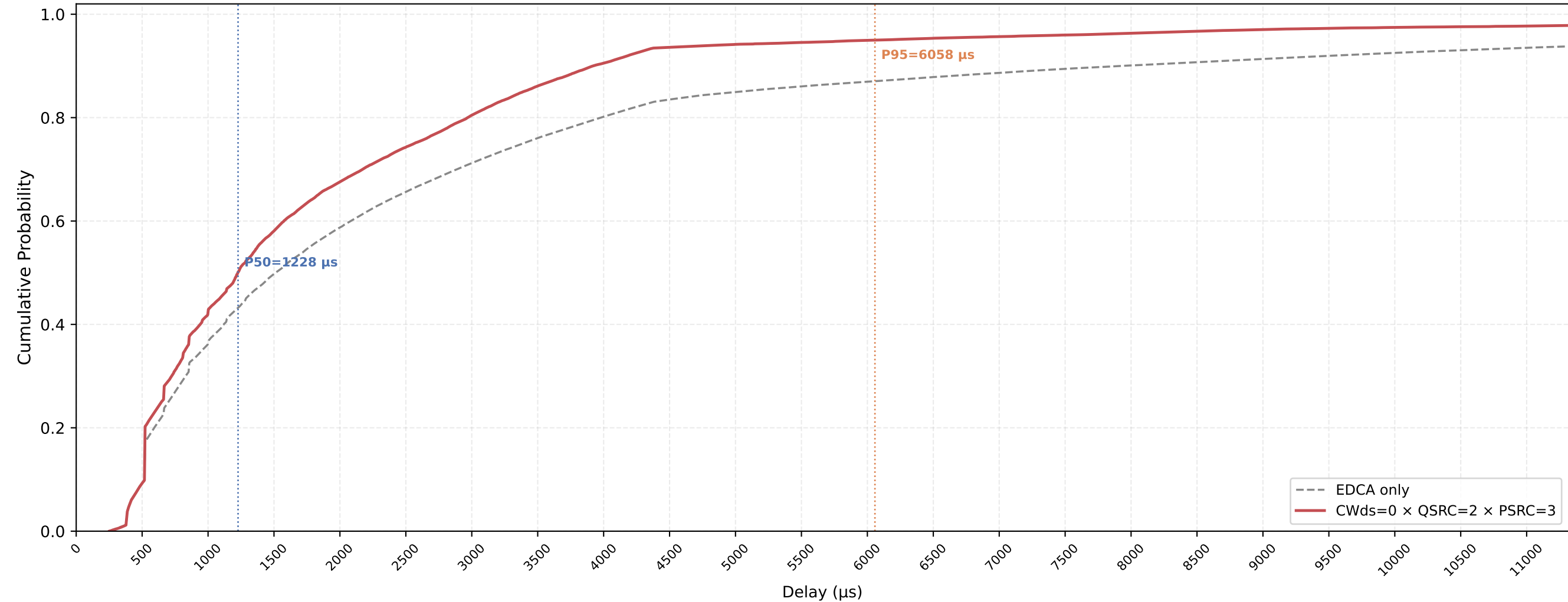
P-EDCA STA VO Delay CDF — CWds=0 × QSRC=2 × PSRC=3 nSta=30, nPedca=5, 1Mbps, avg of 10 runs
