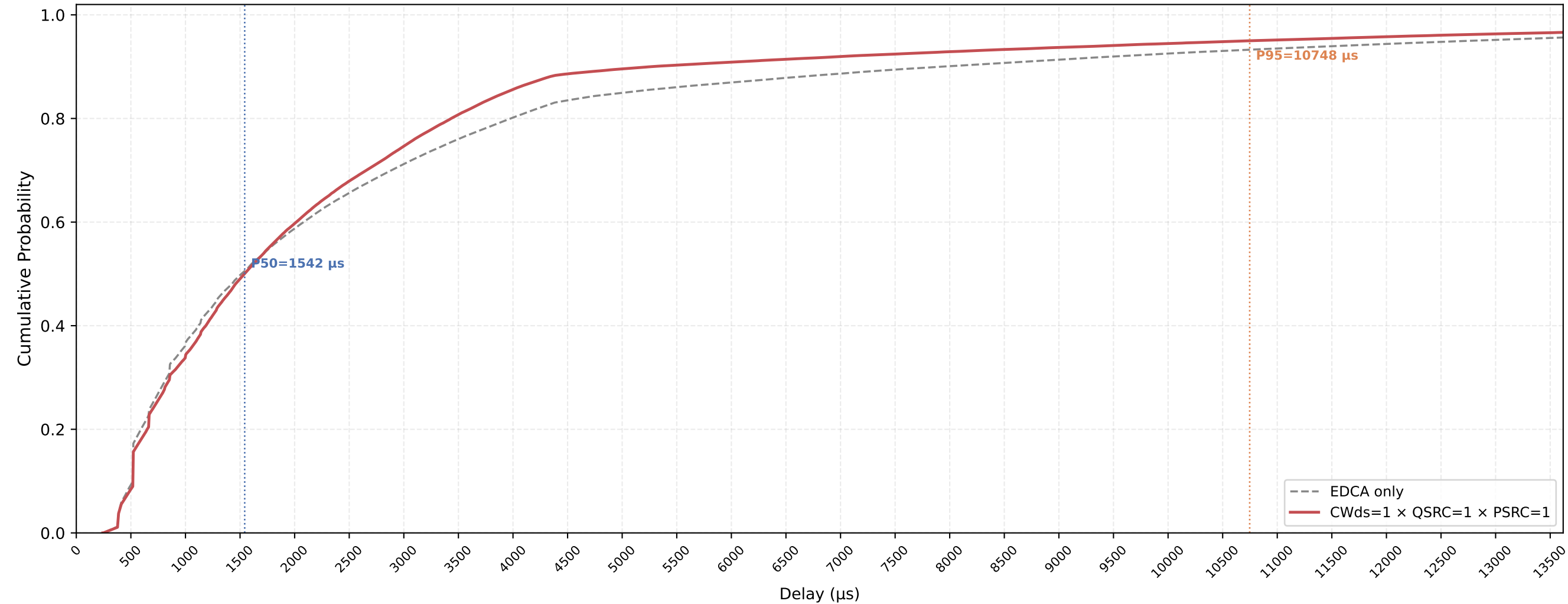
P-EDCA STA VO Delay CDF — CWds=1 × QSRC=1 × PSRC=1 nSta=30, nPedca=15, 1Mbps, avg of 10 runs
